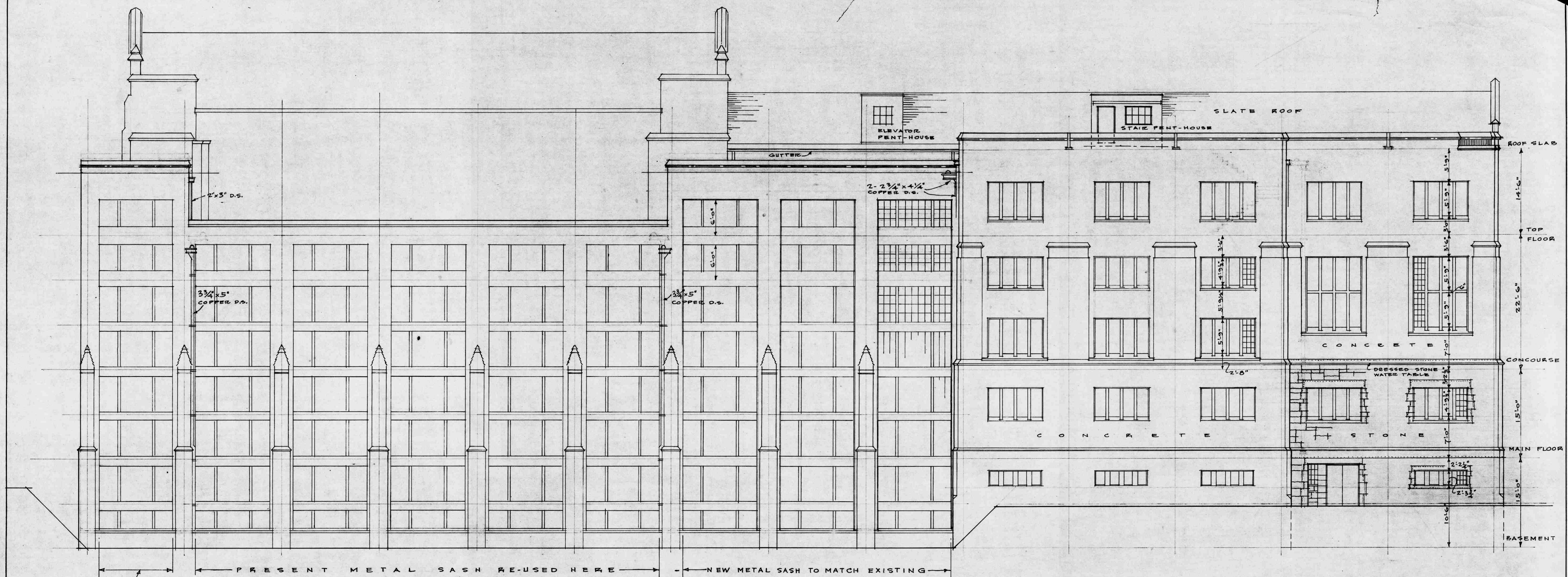
REAR (EAST) ELEVATION
