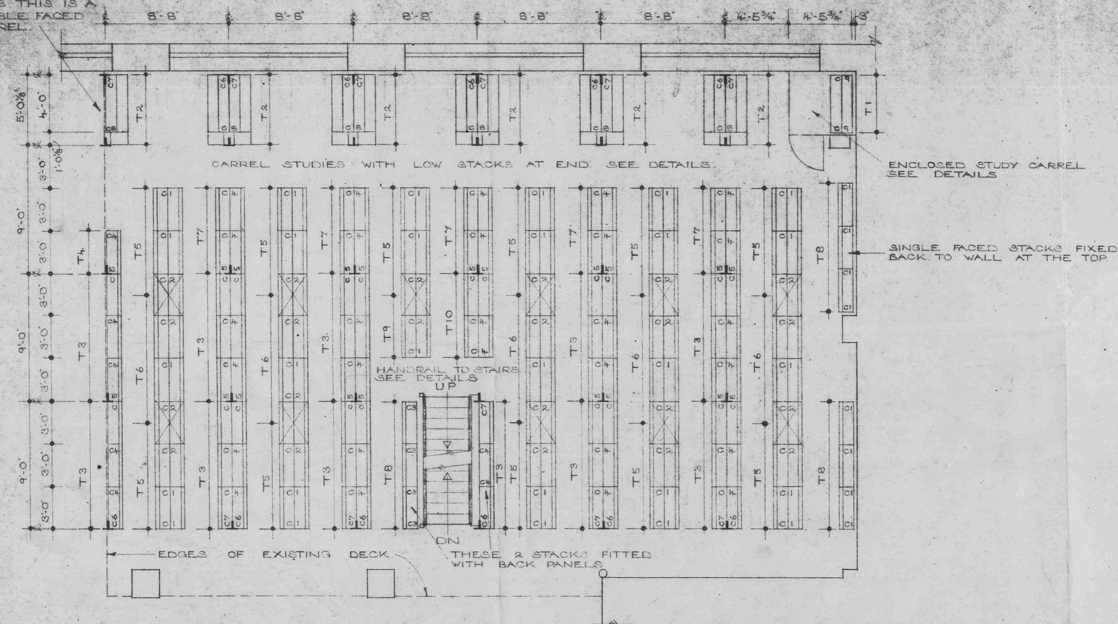
LAYOUT OF STACKS TO LEVELS 1-2-3 & 6
