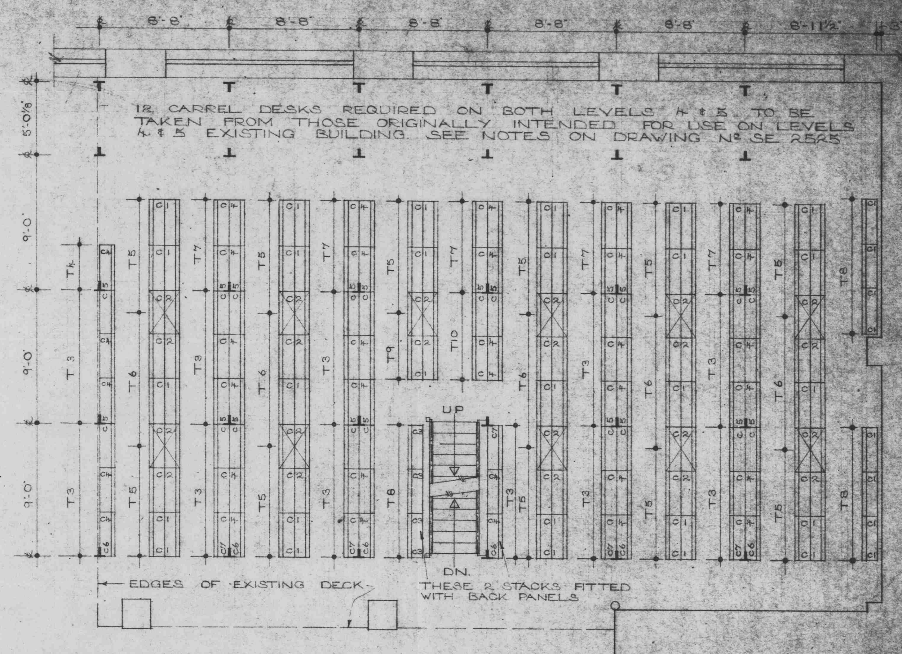
LAYOUT OF STACKS TO LEVELS 4 & 5
