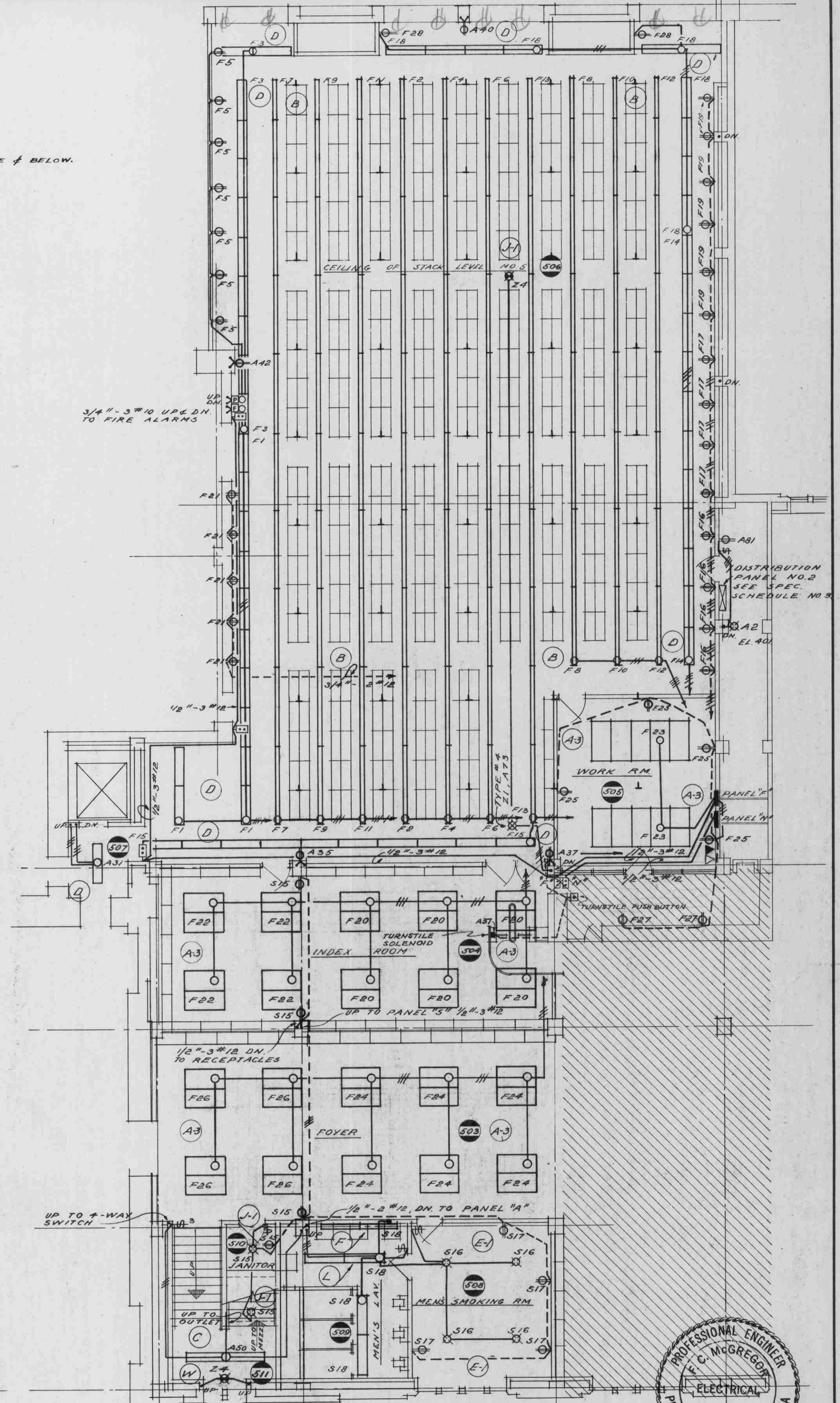
CEILING PLAN OF STACK LEVEL NO. 5
