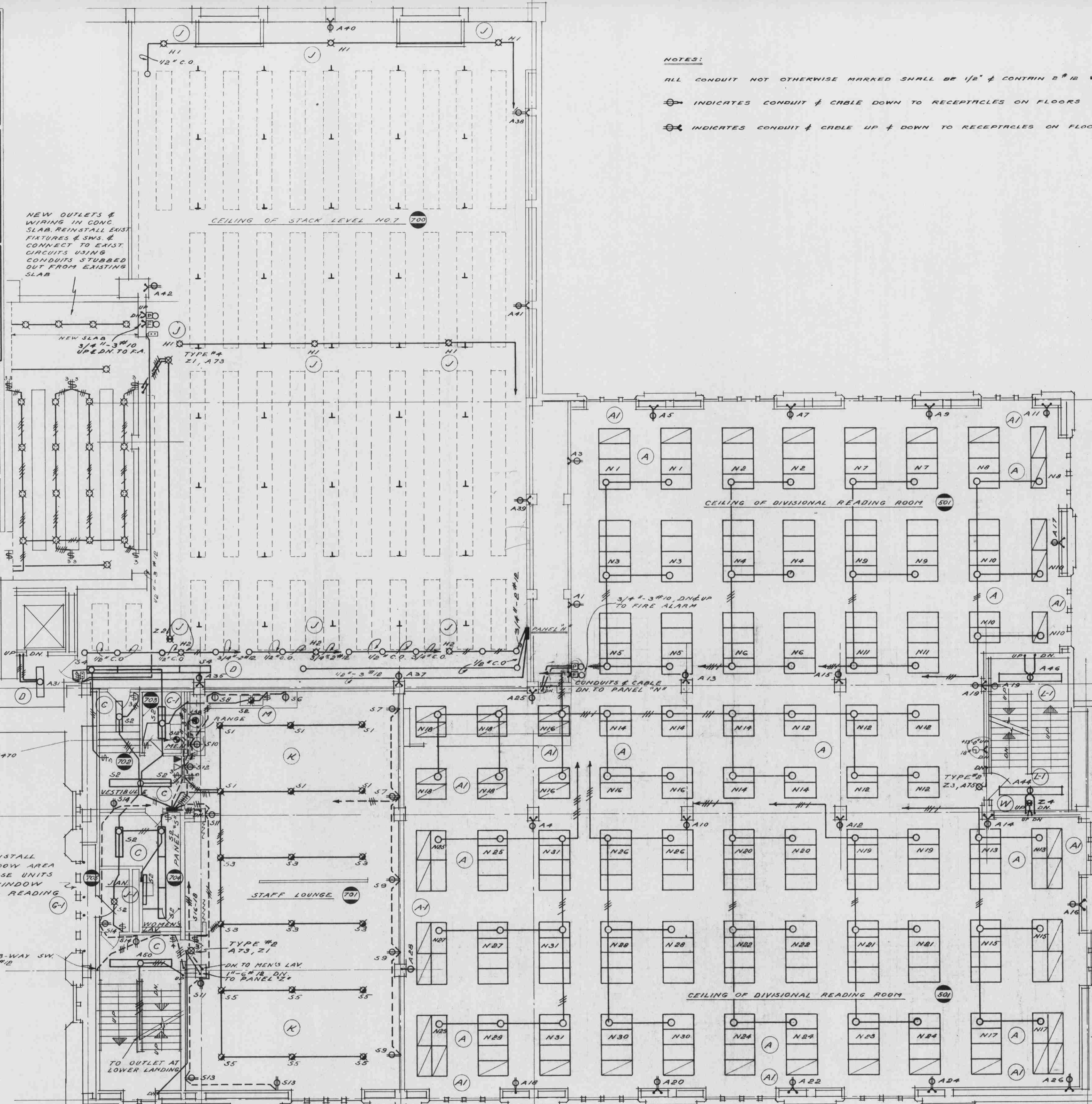
CEILING PLAN OF STACK LEVEL NO. 7
