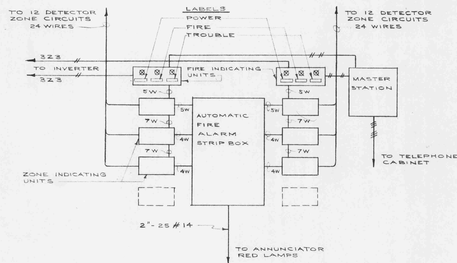
DIAGRAM OF AUTOMATIC DETECTOR UNIT
