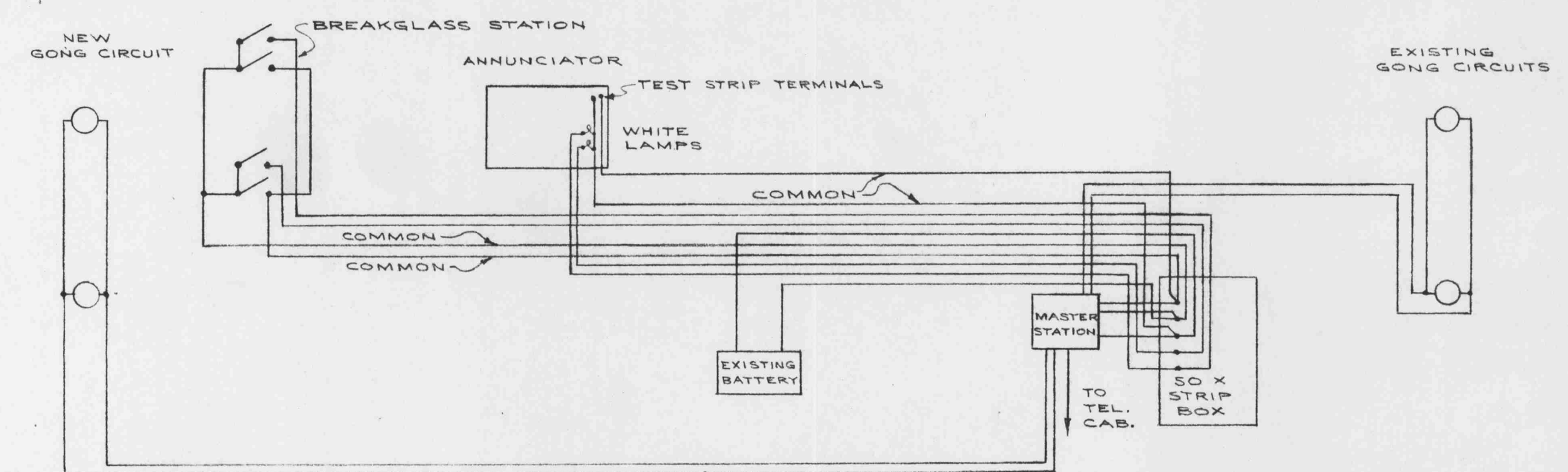
TYPICAL WIRING DIAGRAM FOR MANUAL FIRE ALARM SYSTEM
