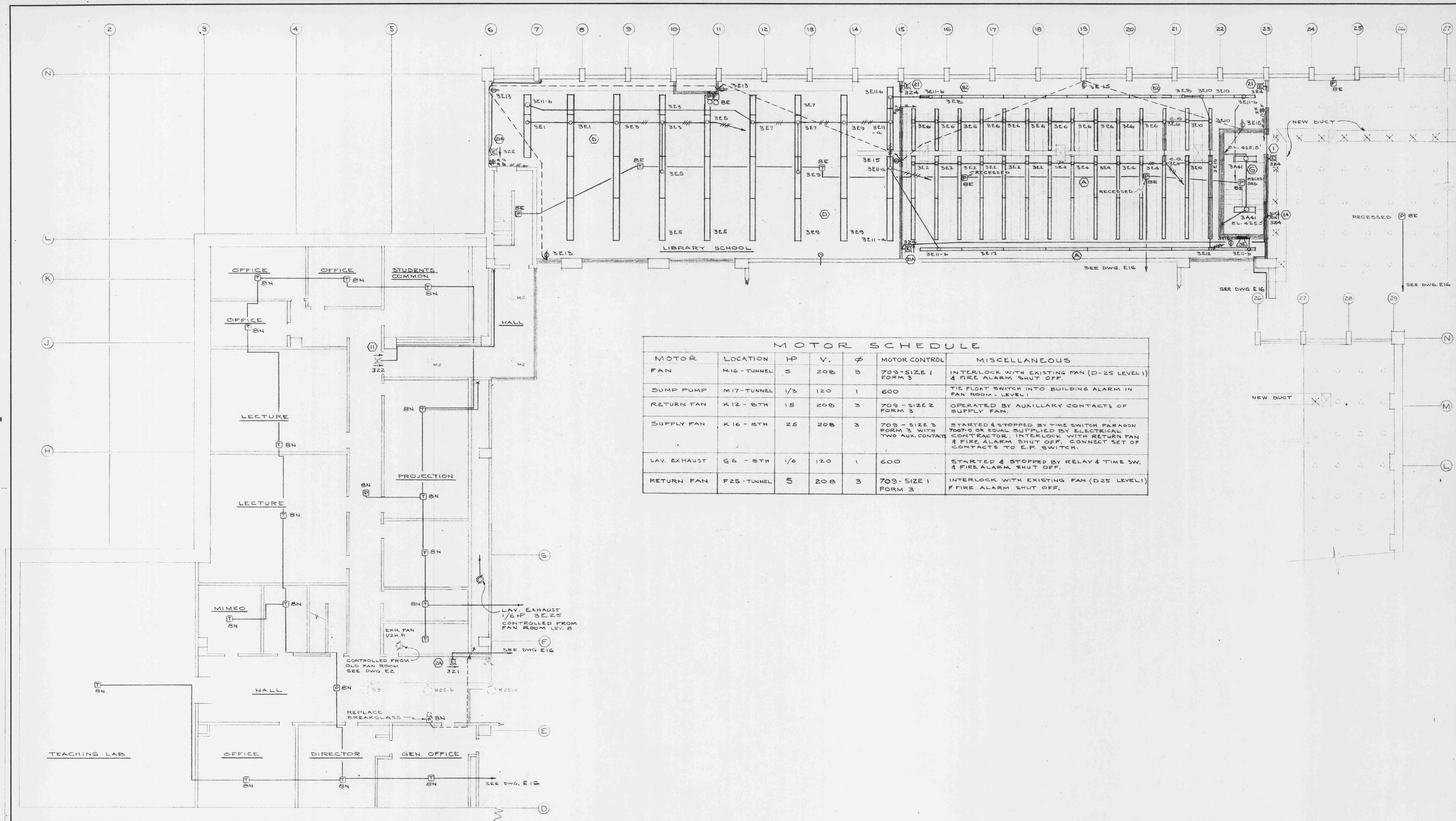
FLOOR PLAN - LEVEL NO. 8 N.E.
