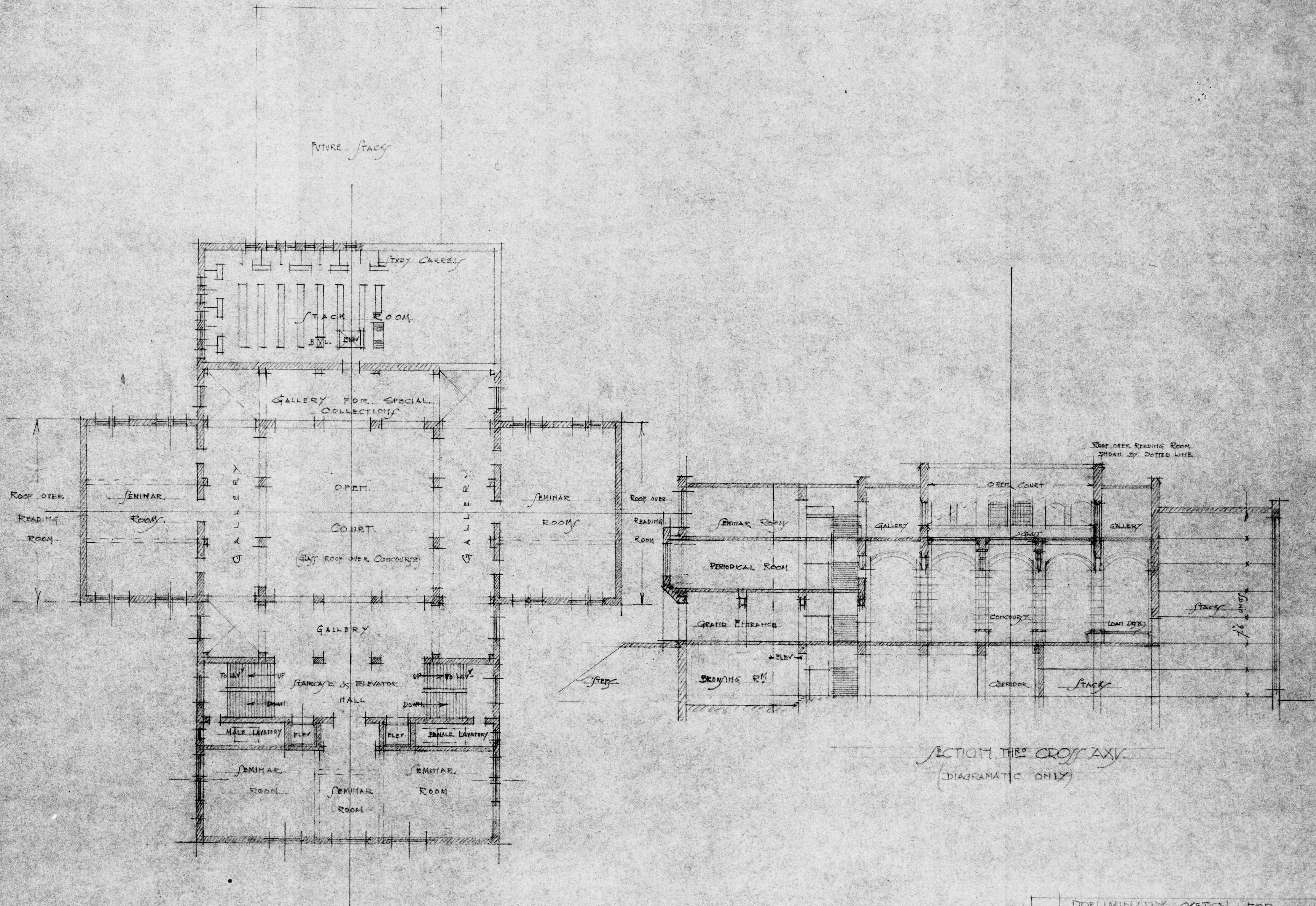
TOP FLOOR PLAN (ULTIMATE LAYOUT)
