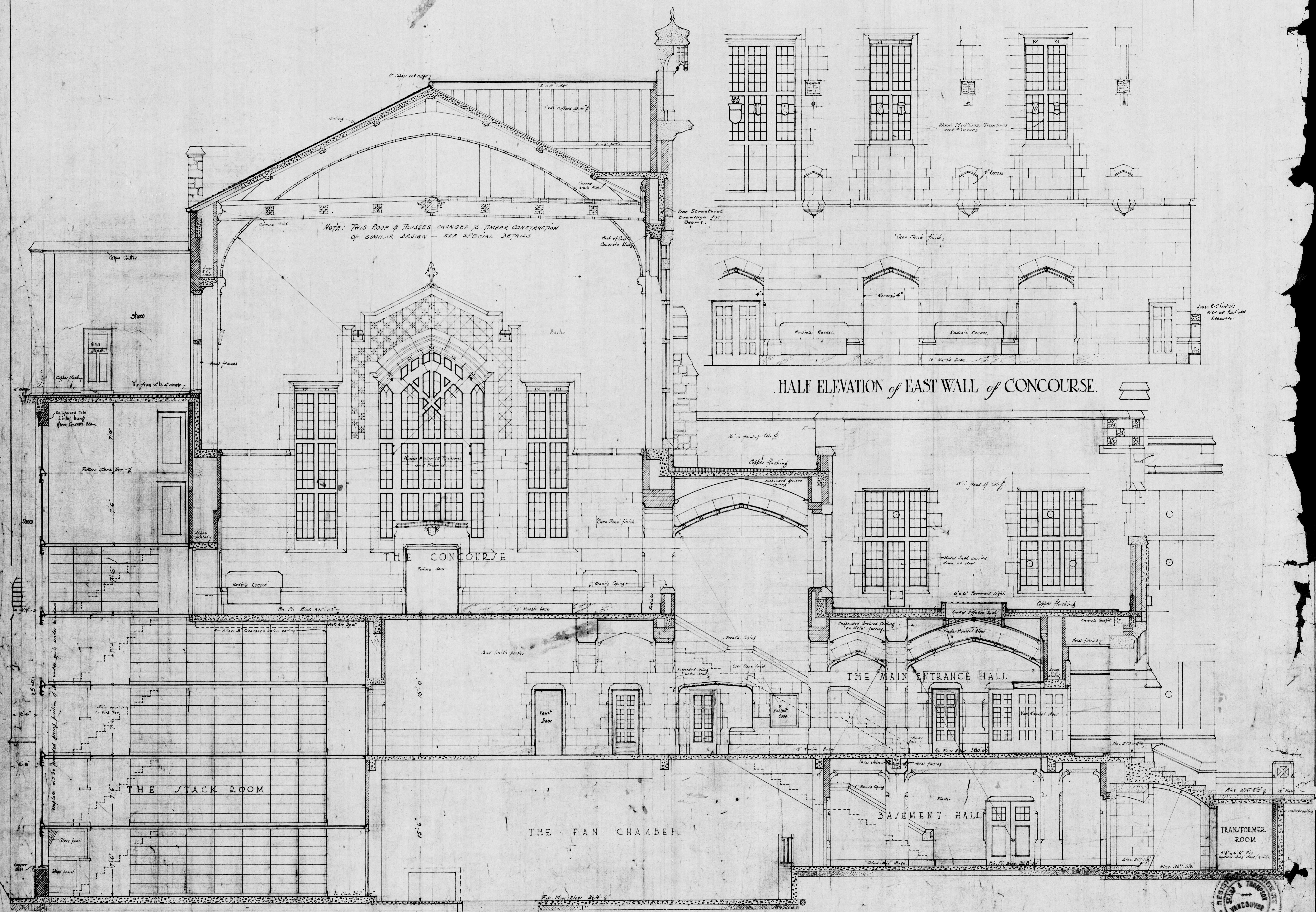
CROSS SECTION thro' center line of building
