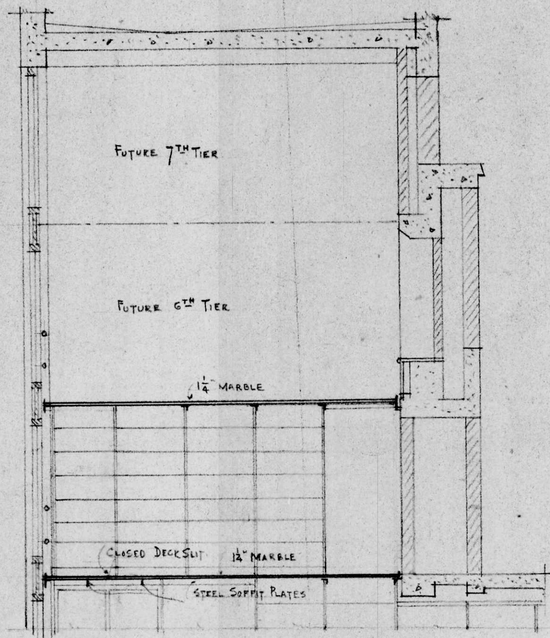
SECTION ON LINE B-B
