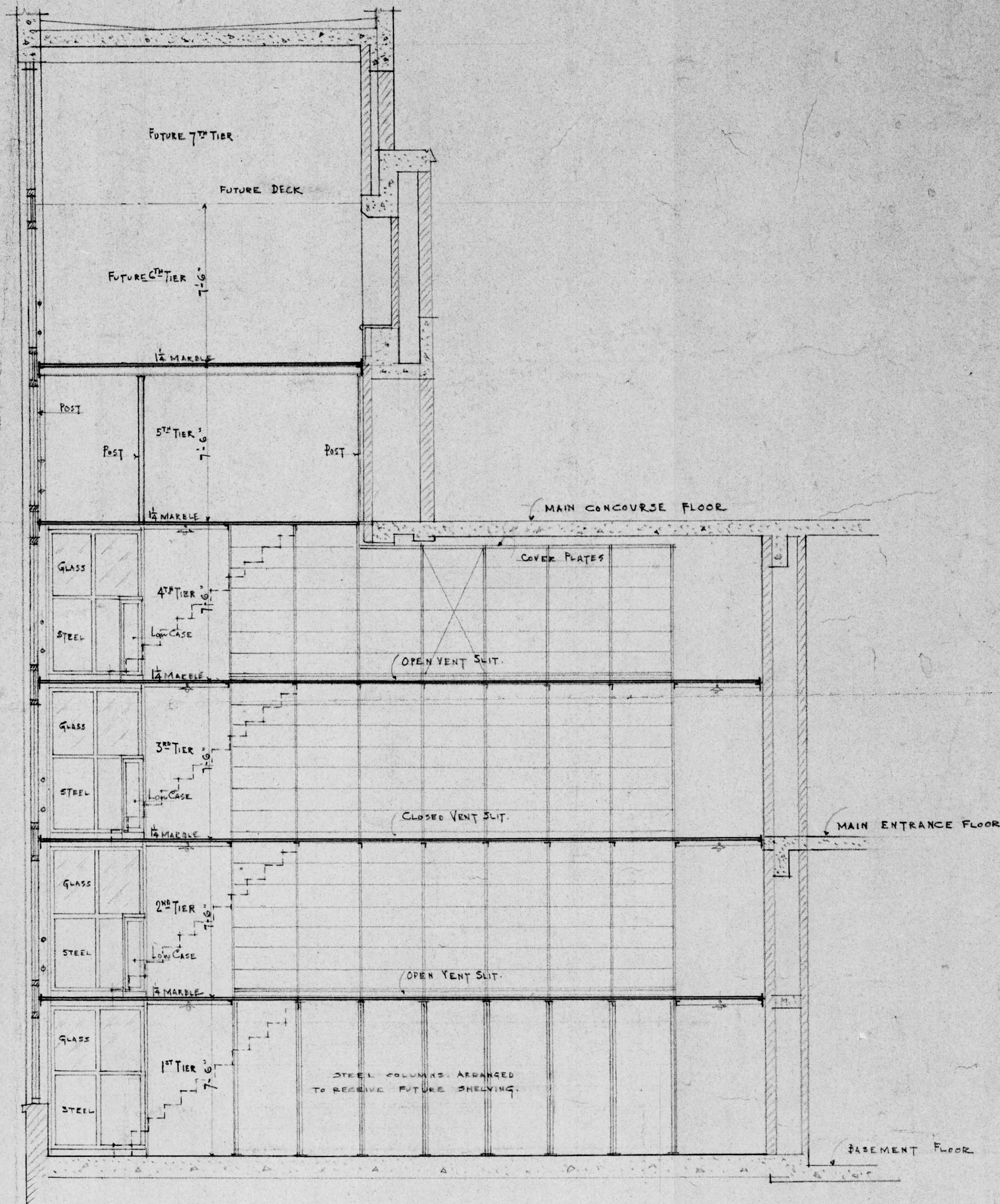
SECTION ON LINE A-A
