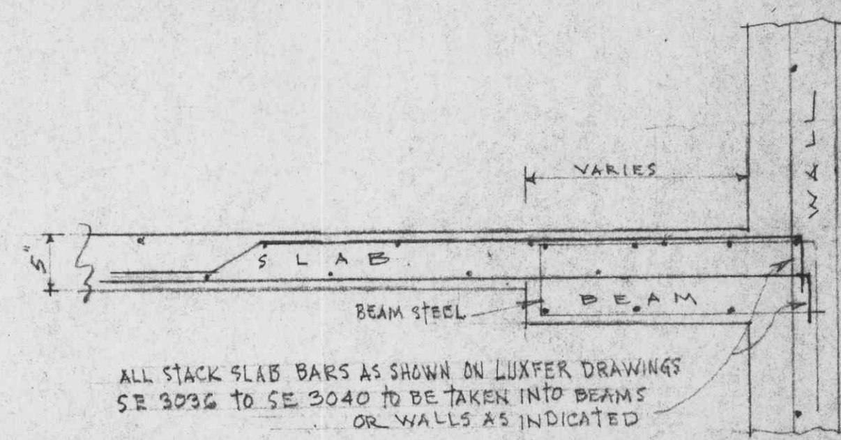
MONOLITHIC SLAB CONNECTION TO NEW WORK
