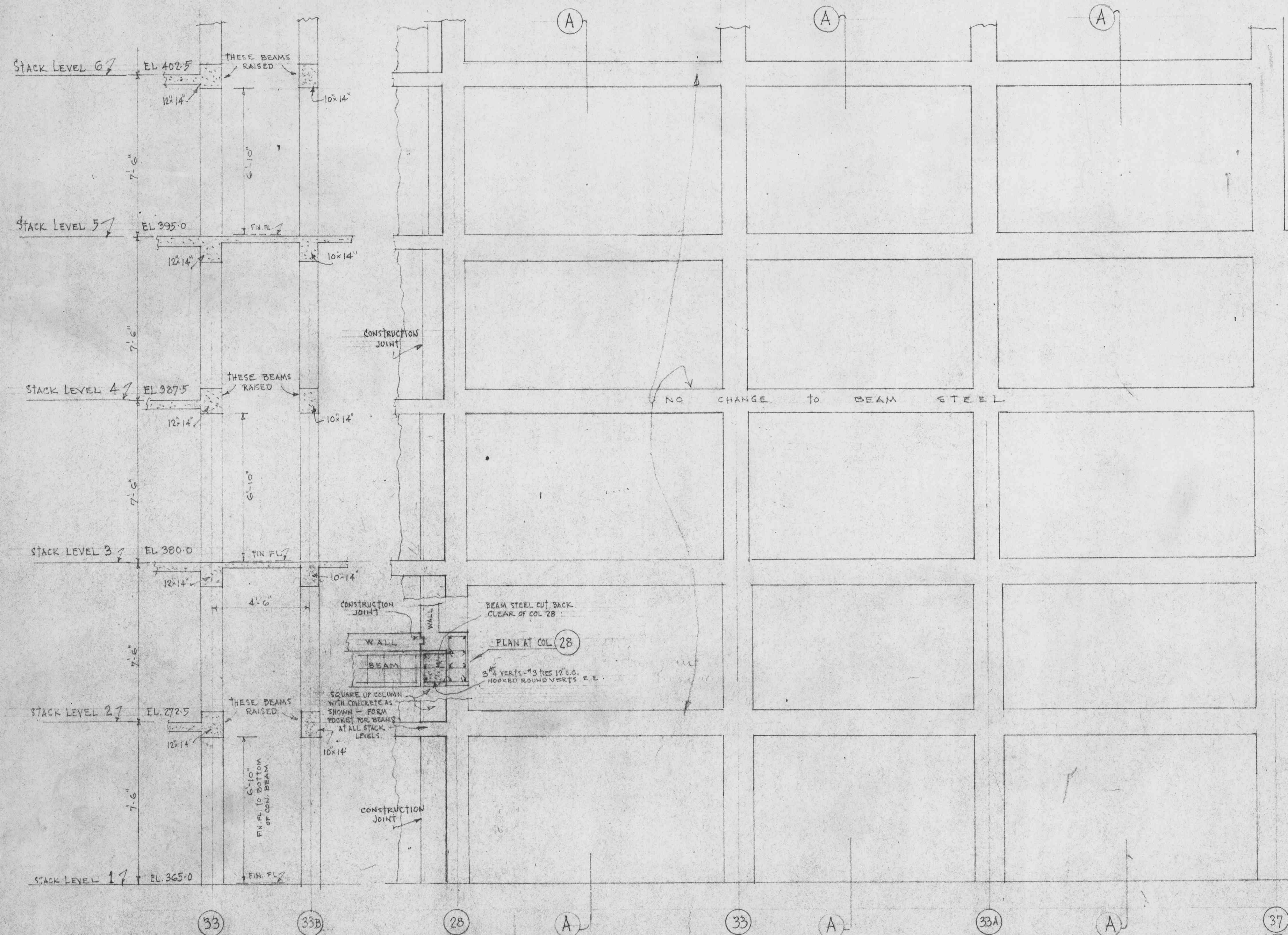
SECTION AT A-A LOOKING SOUTH
