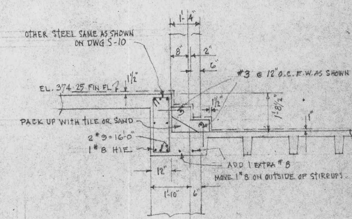
REVISED SECTION A-A OF DRAWING S-2 SCALE \frac{3}{8}'' = 1'-0''
