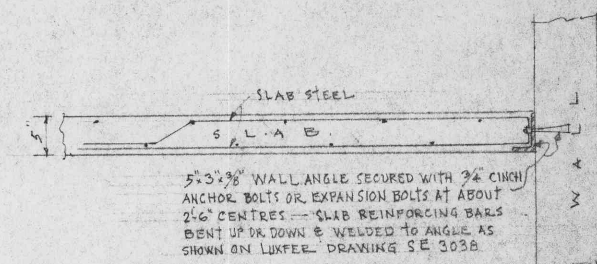
MONOLITHIC SLAB CONNECTION TO EXISTING WORK
