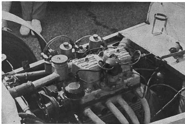
⬆ The Ford 100 E-modified engine in Zelma's car.
