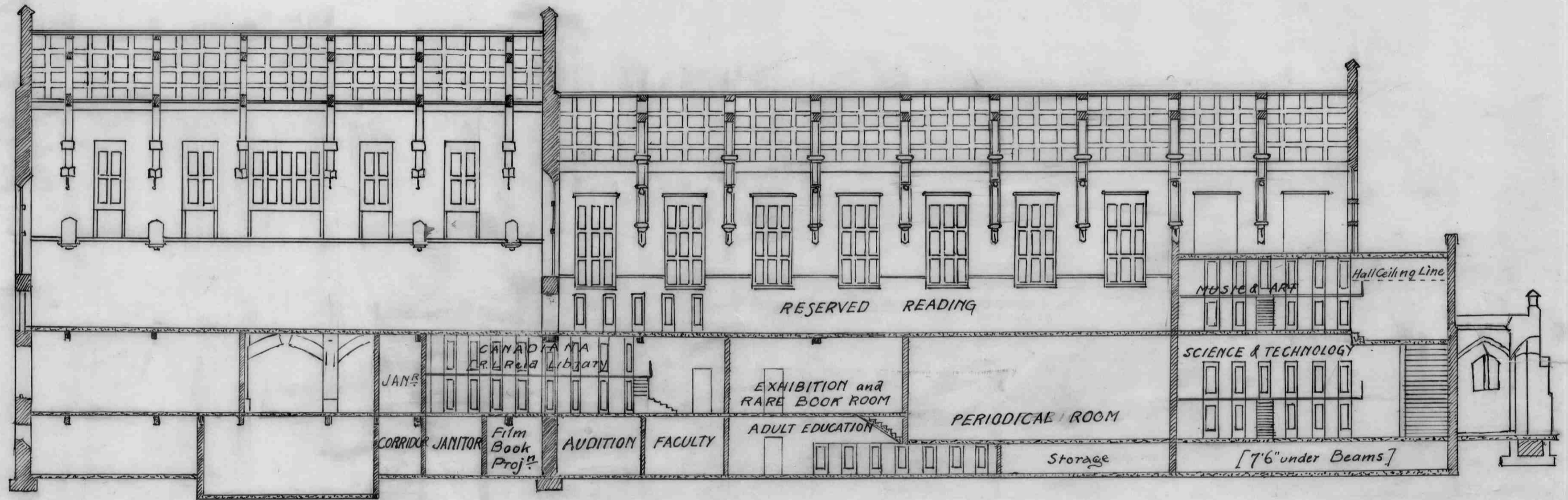
TRAN LONGITUDINAL SECTION.
