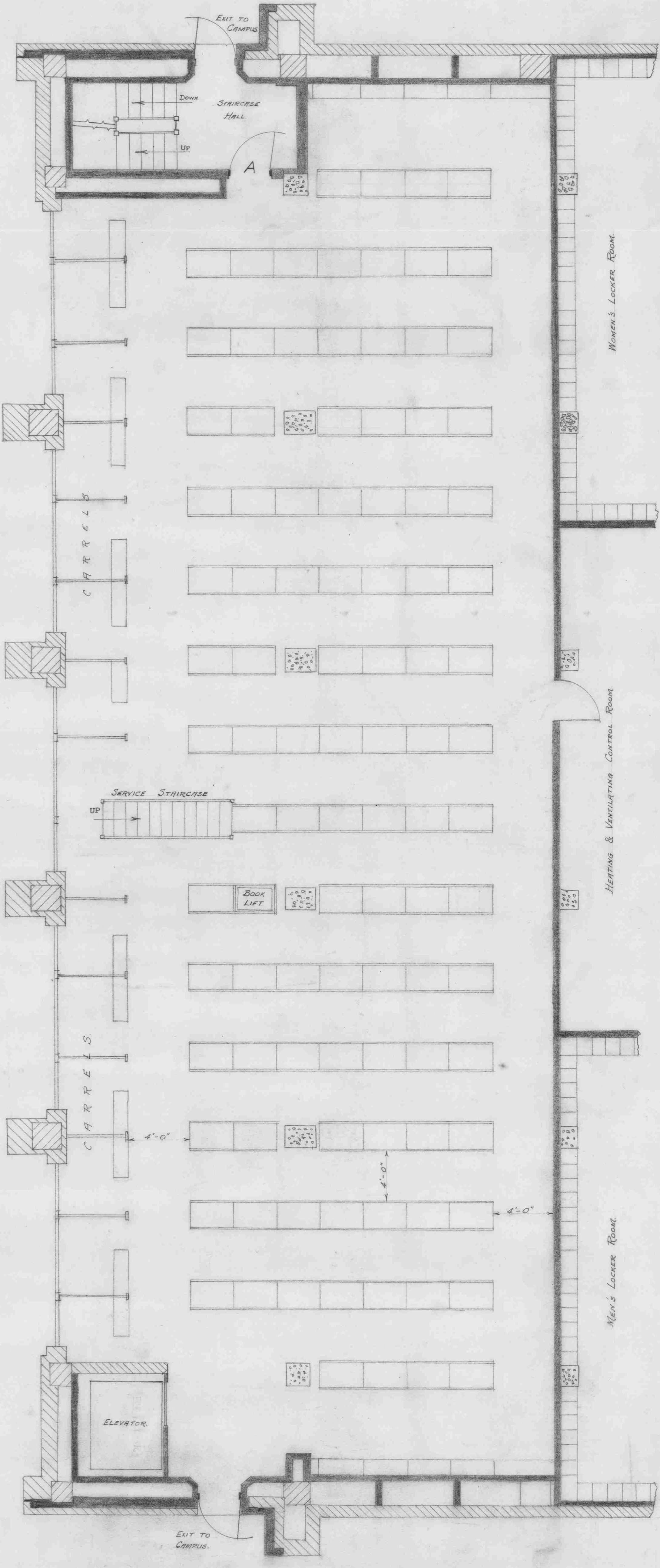
— THE LIBRARY — THE UNIVERSITY OF BRITISH COLUMBIA. VANCOUVER, B. C., CANADA STACK ROOM SYSTEM PLAN OF TIER 1 BASEMENT FLOOR
