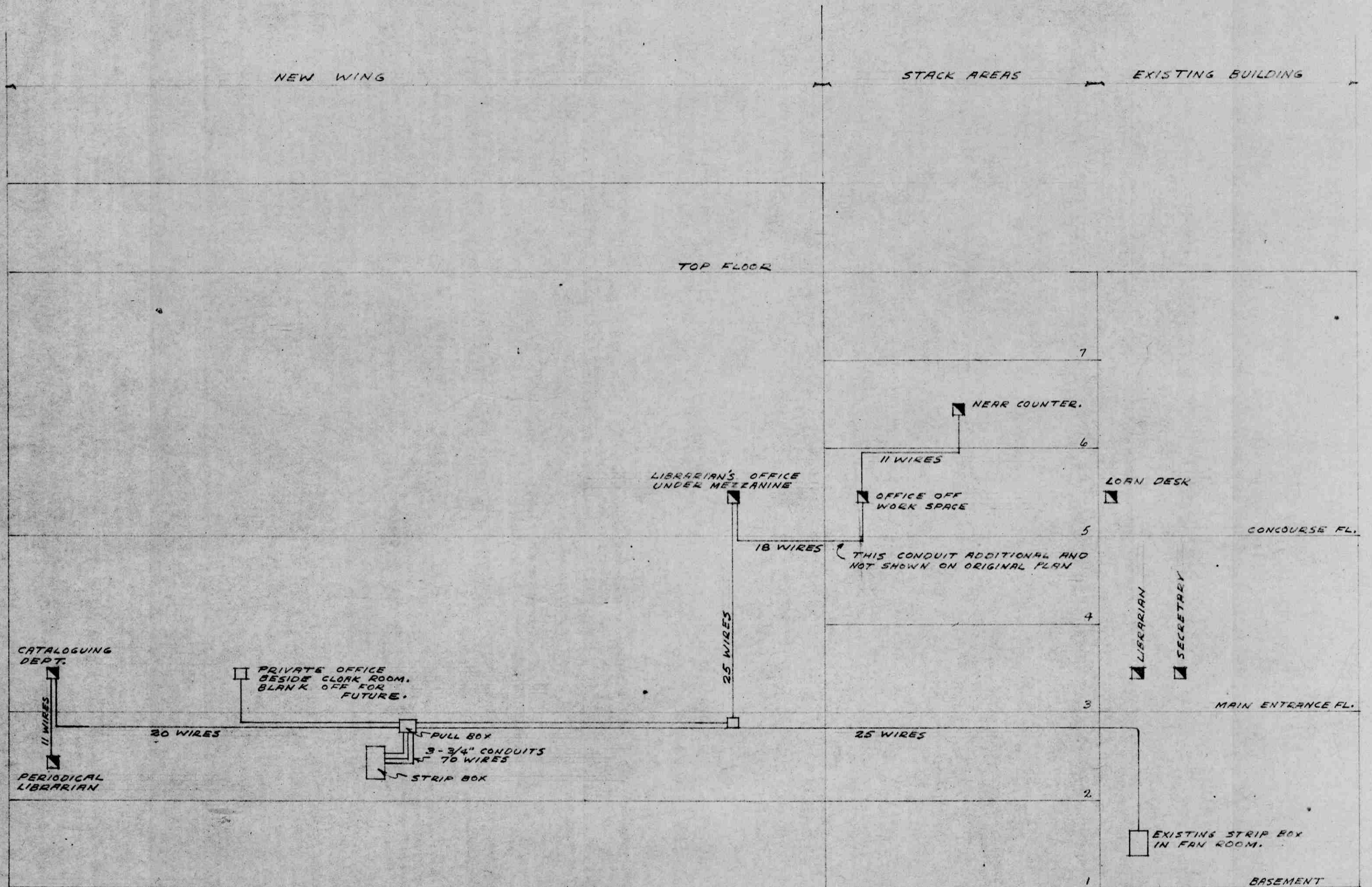
RISER DIAGRAM INTER-COMMUNICATION SYSTEM NOT TO SCALE
