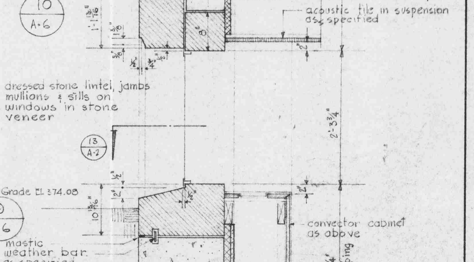
Wall section West Wall Scale 1"=1'-0"
