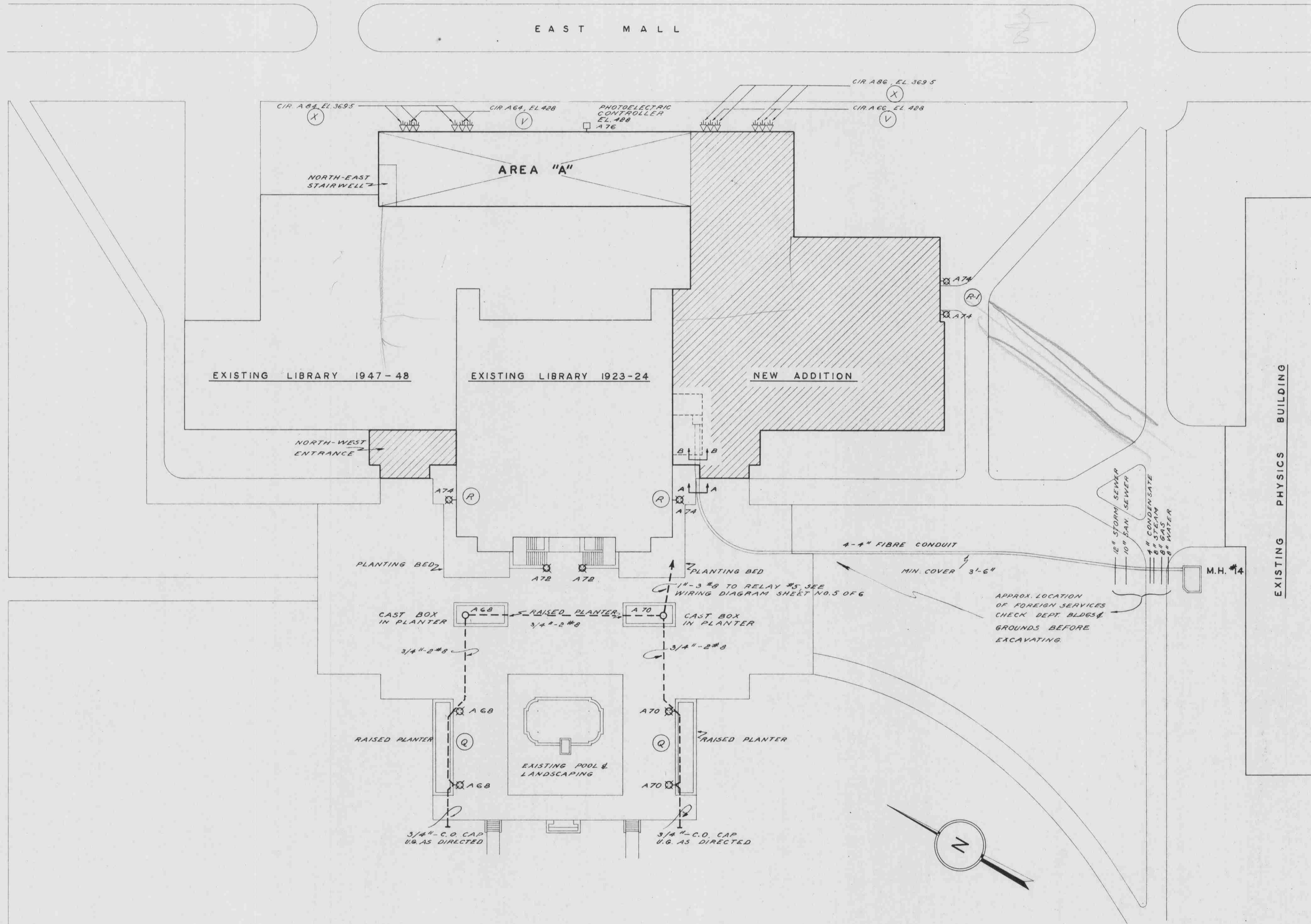
SITE PLAN SCALE: 1" = 30'-0"
