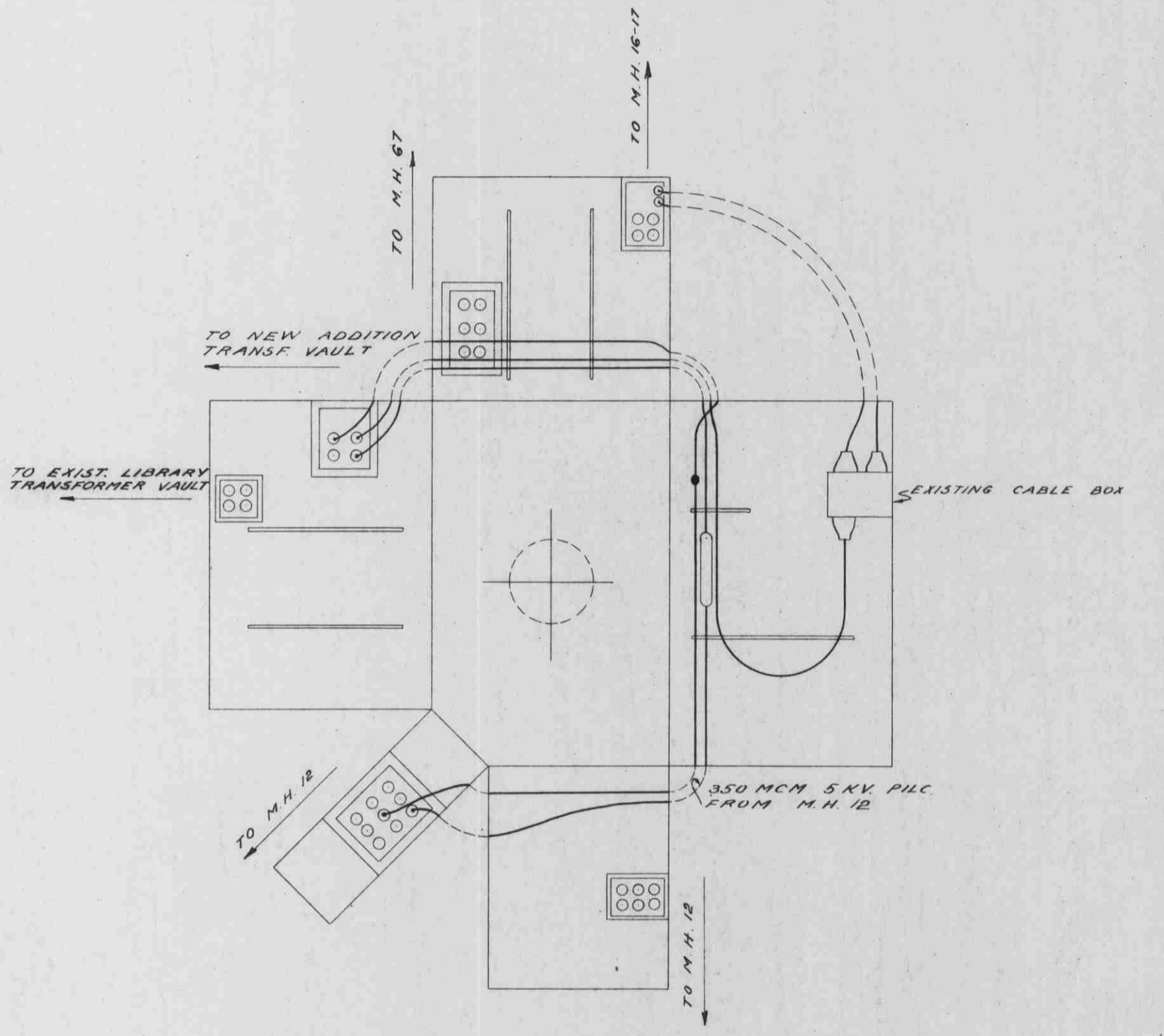
DEVELOPMENT PLAN OF MANHOLE #14 SCALE: 1/4" = 1'-0"
