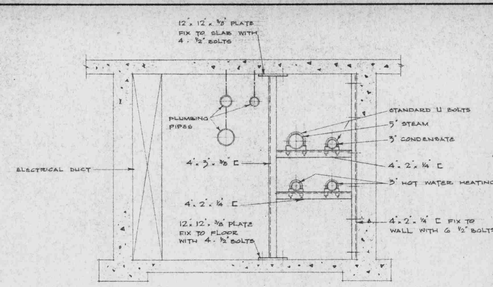
DETAIL OF PIPE ANCHOR IN TRENCH SCALE: 1/2" = 1'-0"
