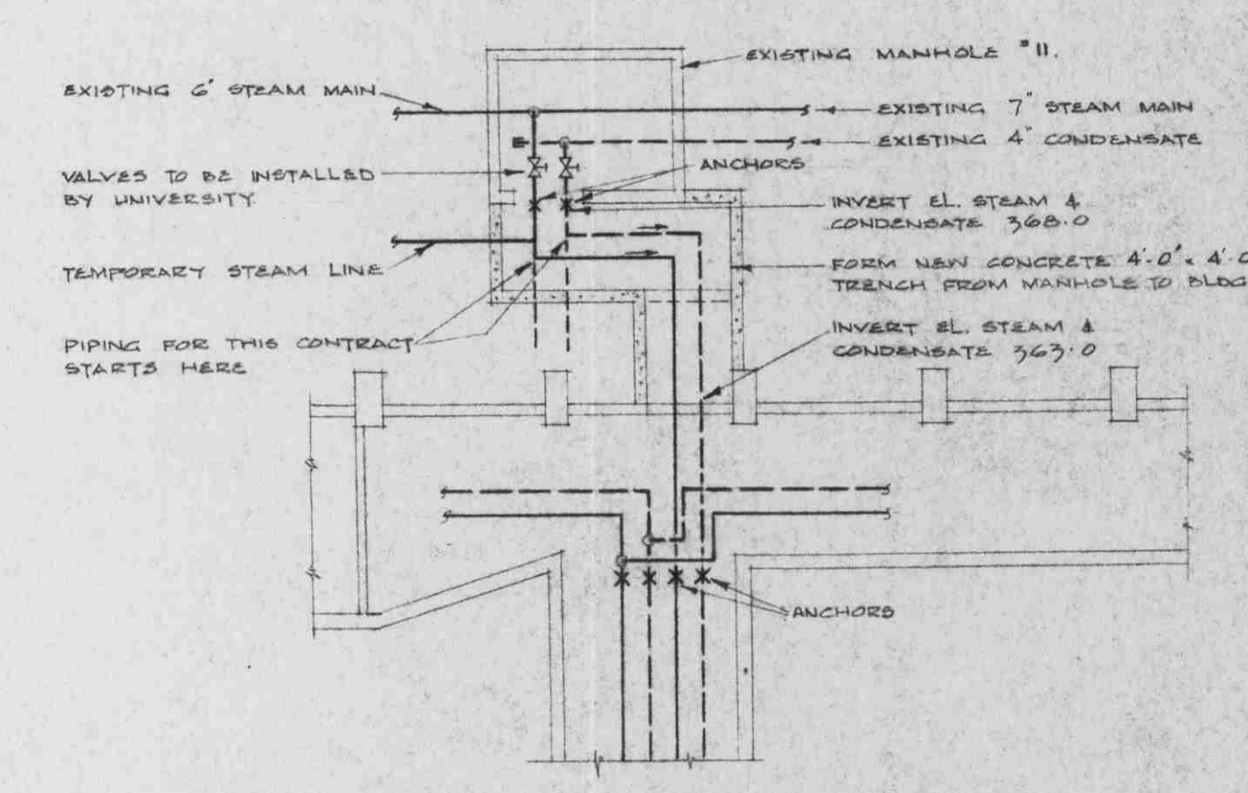
PLAN OF STEAM ENTRY SCALE: 1/8" = 1'-0"
