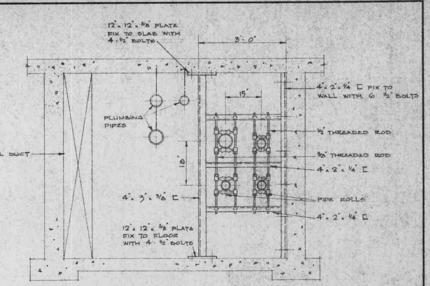
DETAIL OF PIPE GUIDES IN TRENCH SCALE: 1/2" = 1'-0"
