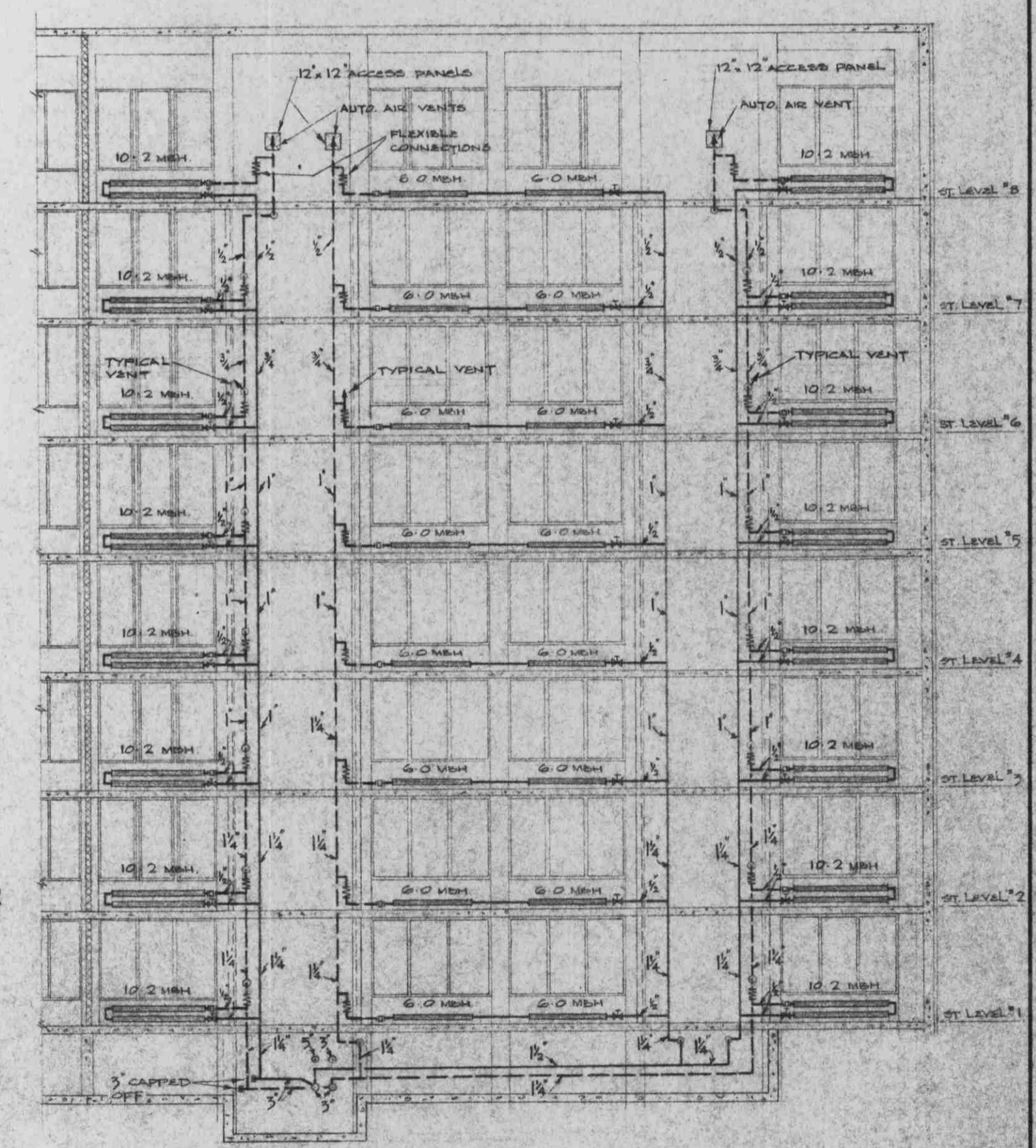
SECTION Y-Y
