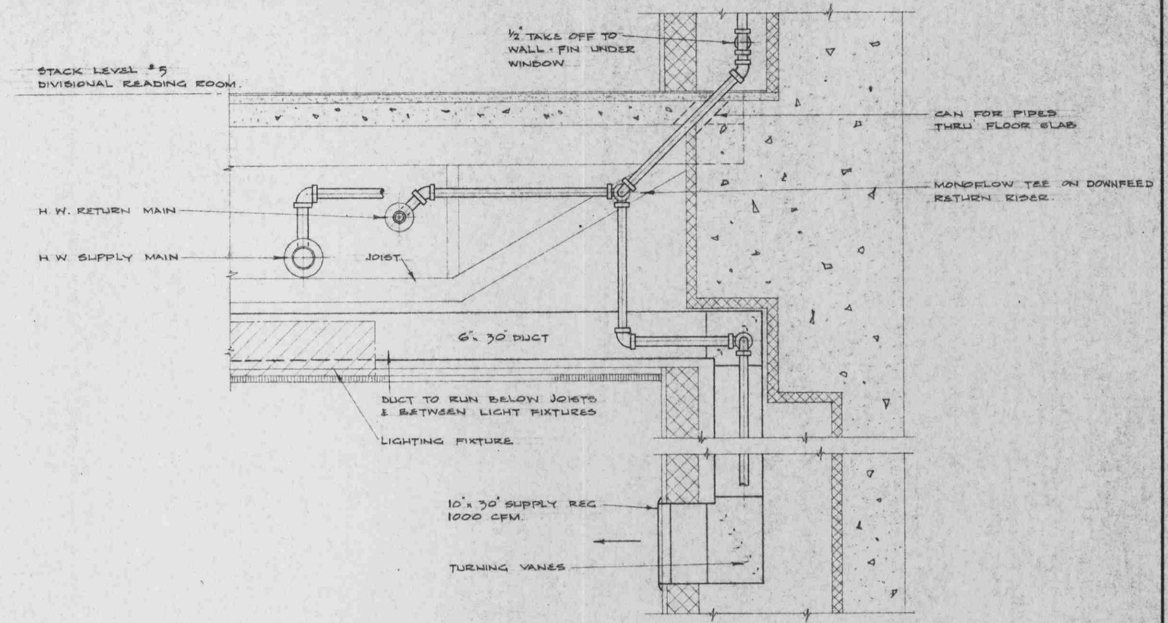
TYPICAL SECTION THRU' COLLEGE LIBRARY #2 CEILING AT OUTSIDE WALLS SCALE: 1" = 1'-0"
