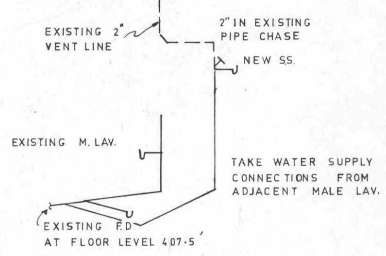
PLUMBING SCHEMATIC FOR SERVICE SINK
