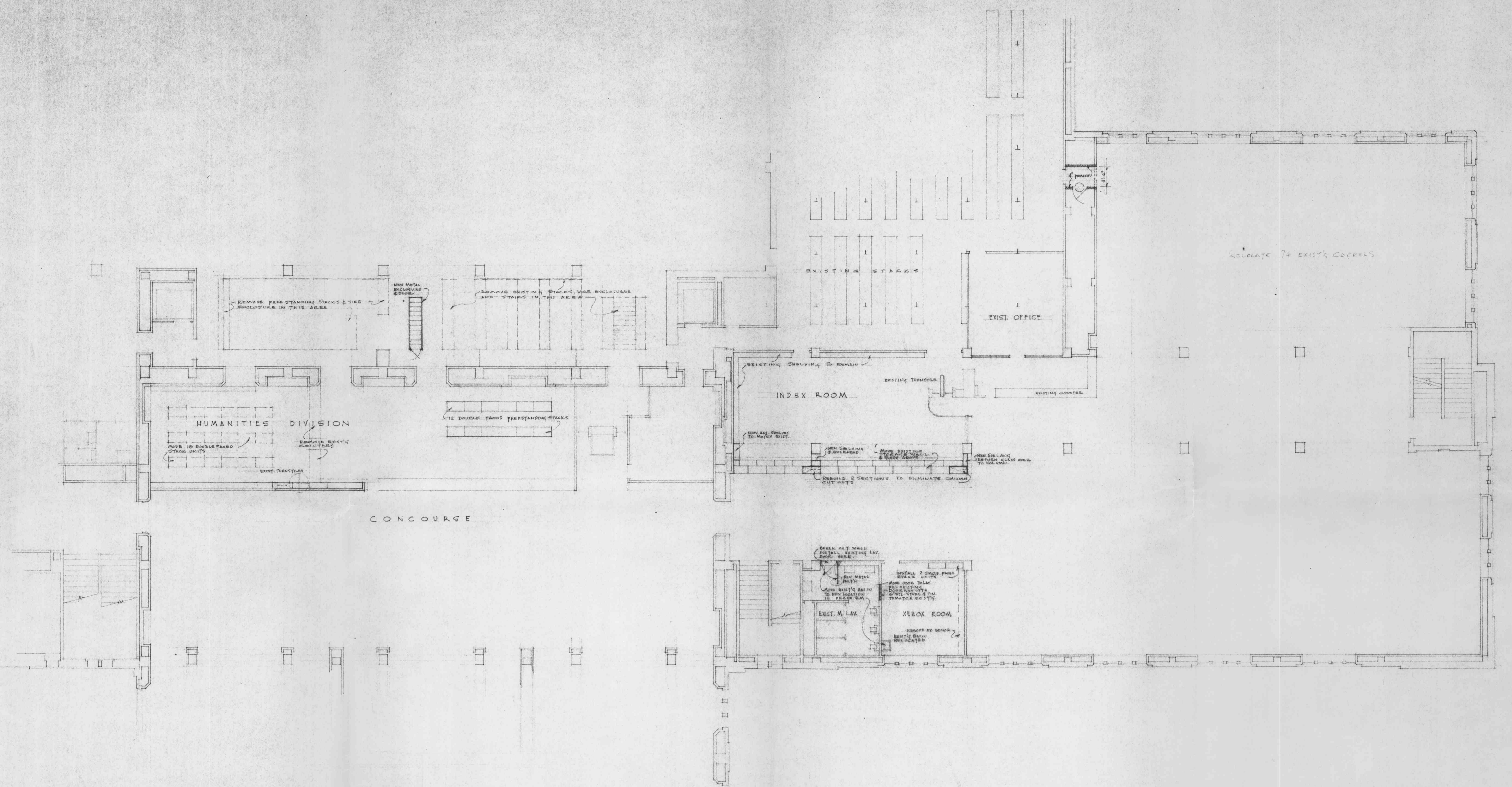
PLAN OF HUMANITIES, SCIENCES & INDEX OFFICES (MAIN CONCOURSE LEVEL NO 5) SCALE 1/8" = 1'-0"
