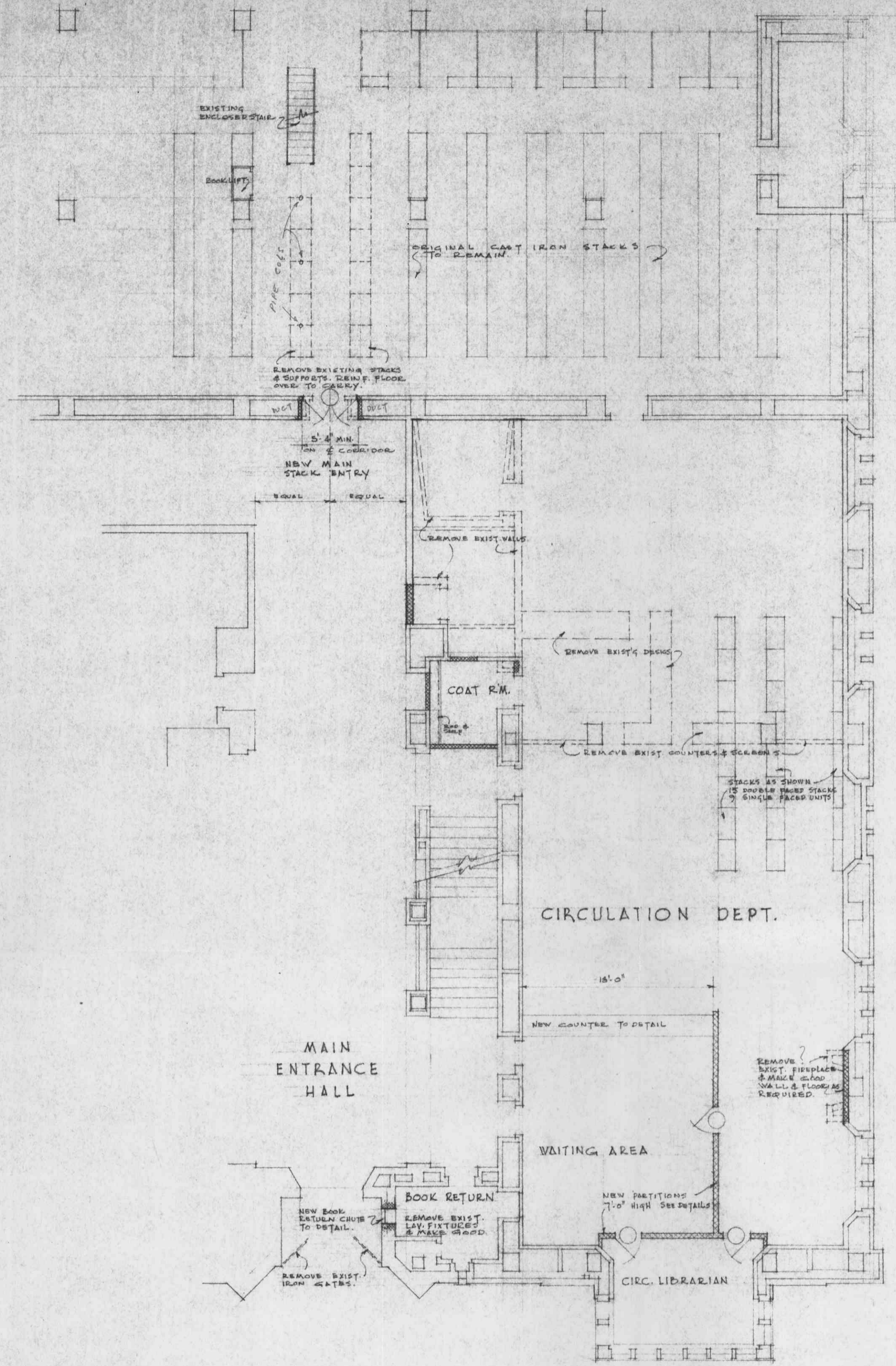
PLAN OF CIRCULATION DEPARTMENT & NEW STACK ENTRY (LEVEL NO. 3) SCALE 1/8" = 1'-0"
