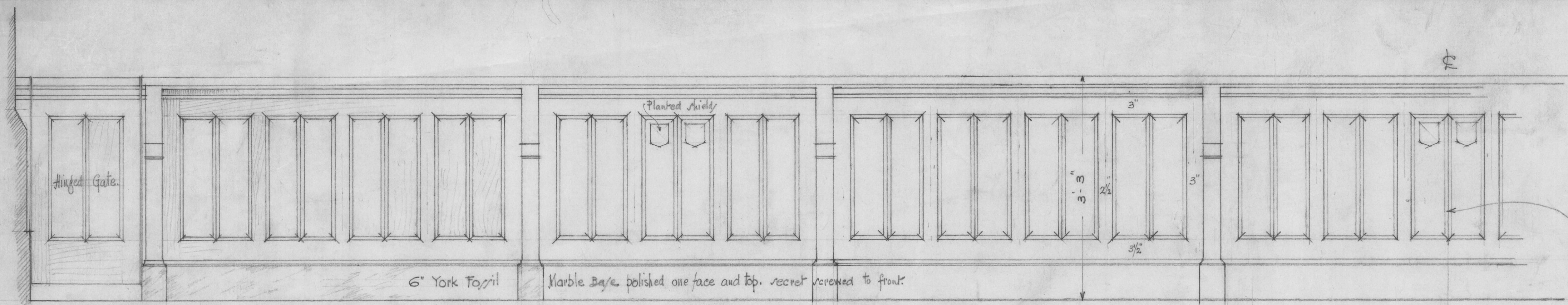
Half Exterior Elevation (developed).
