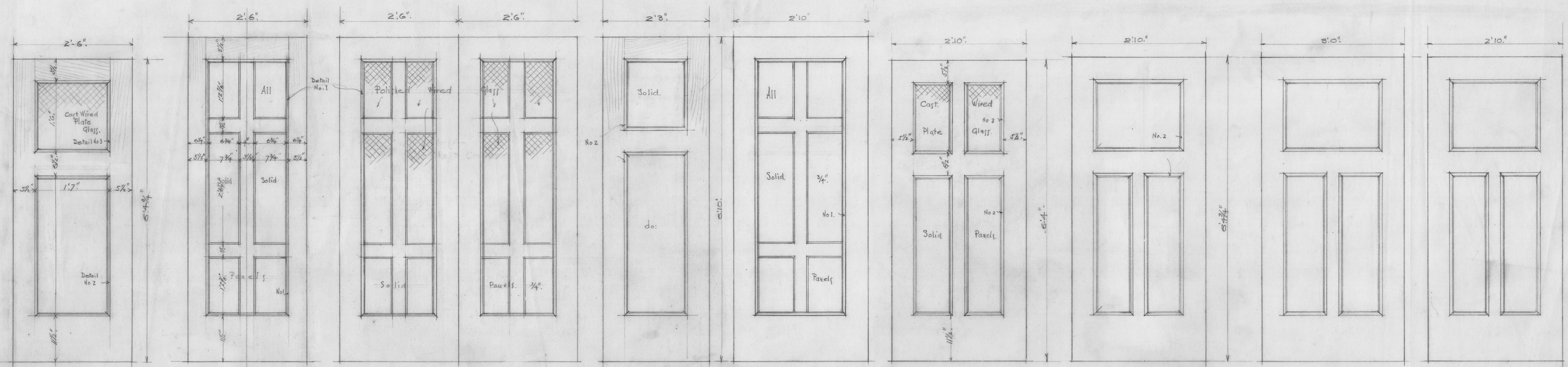
Fire Escape - Stairs. (Seven Req'd.) 2"
