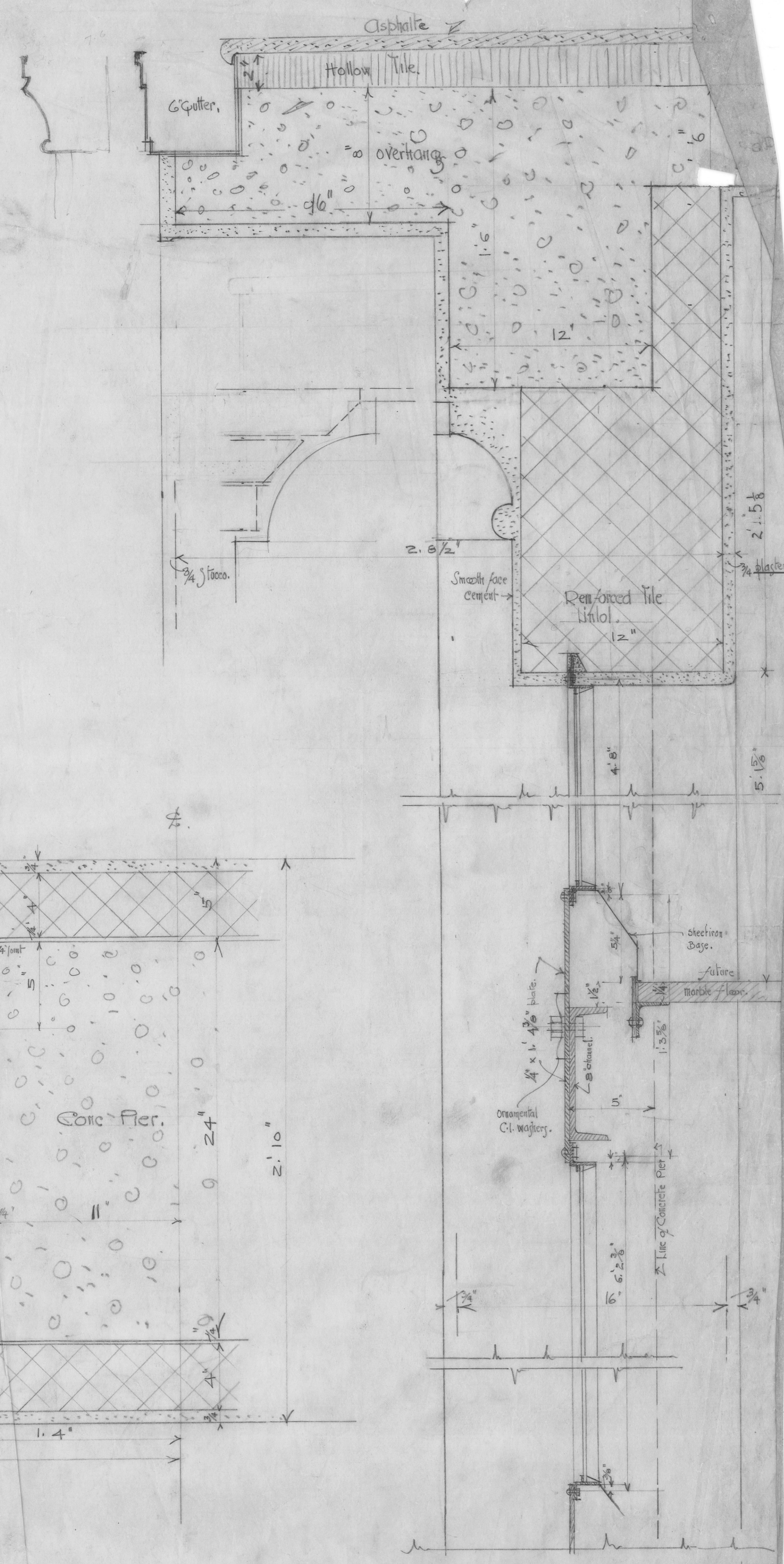
Section of Steel Joist... Bottom Sash, Copper Sill, & Anchor Cement, Tile, Stucco.
