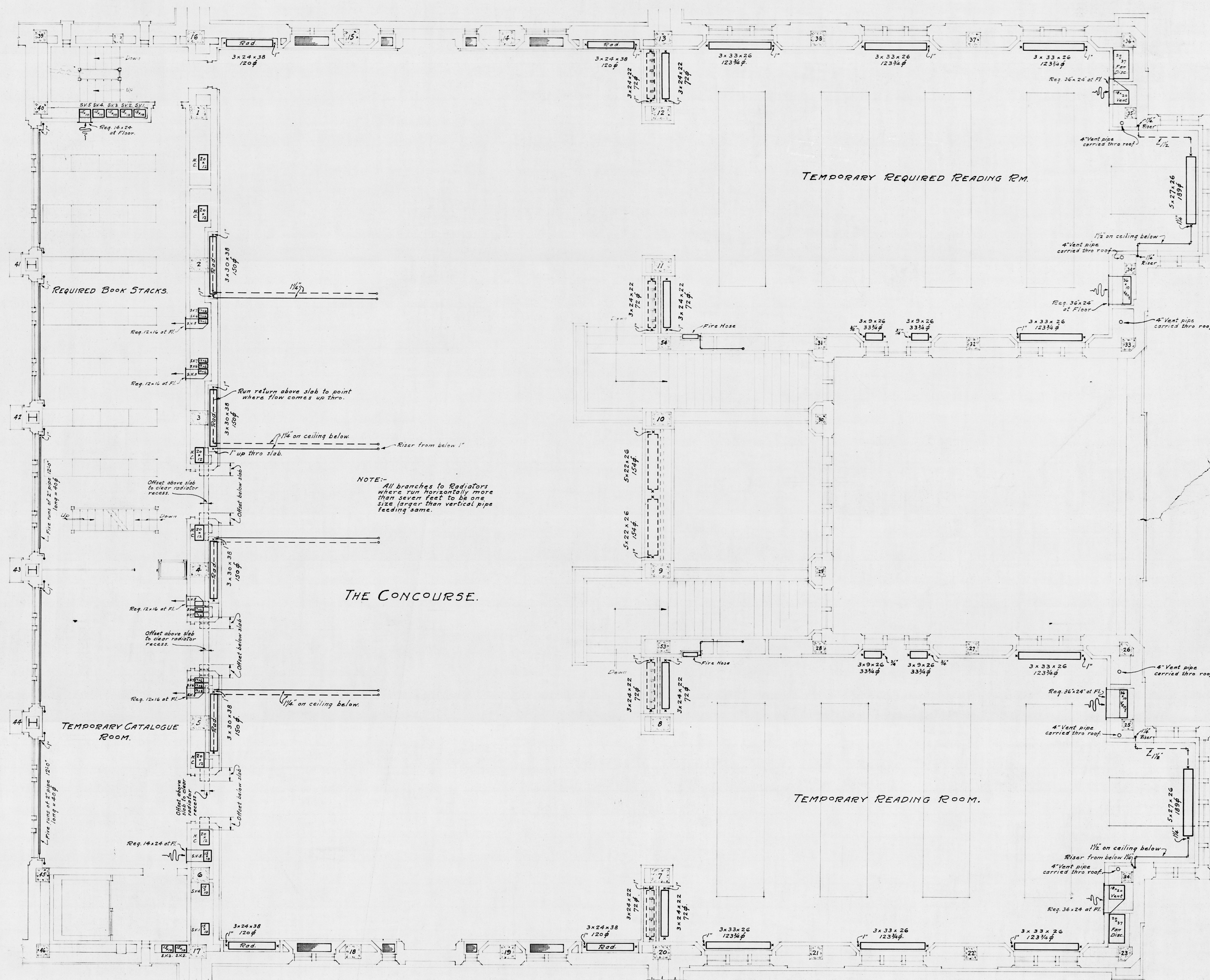
MAIN CONCOURSE FLOOR PLAN.
