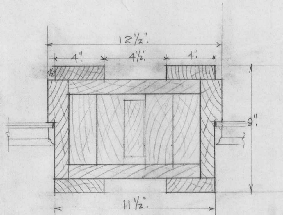
Section of Mullion at A-A.
