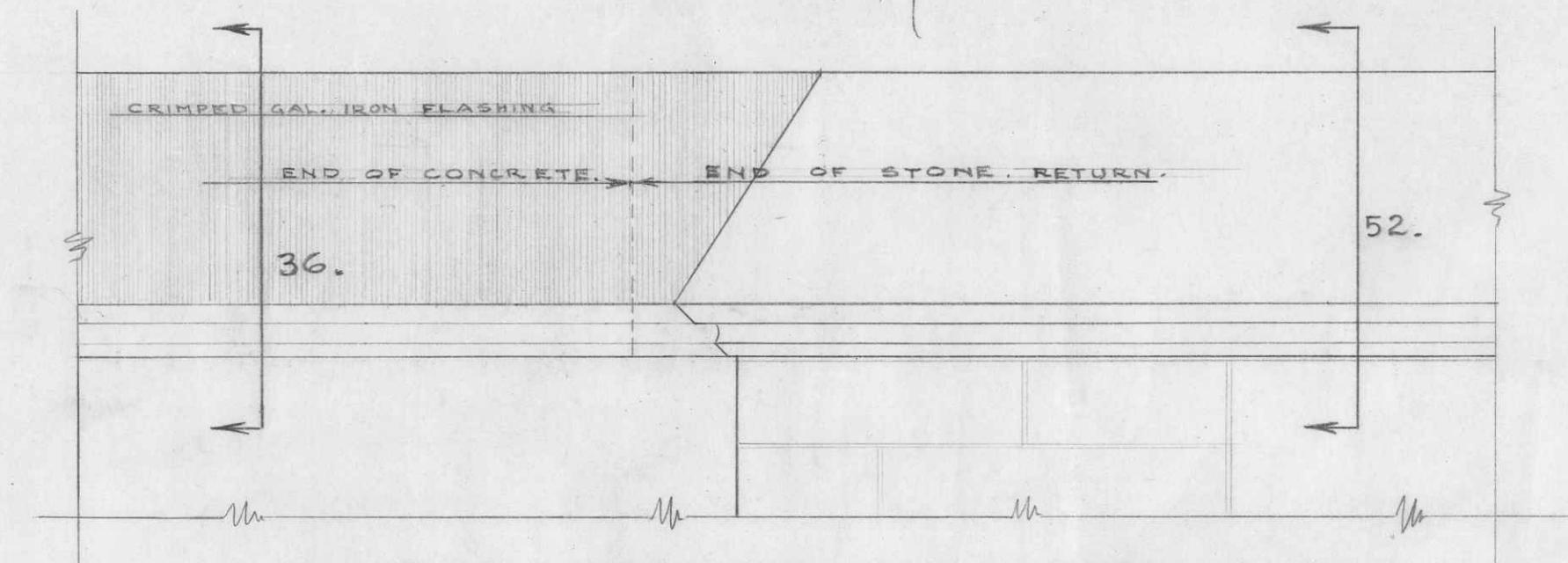
ELEVATION OF COPING SCALE 1/2" = 1'-0" SHOWING JOINING OF CONC. & STONE PARAPETS.
