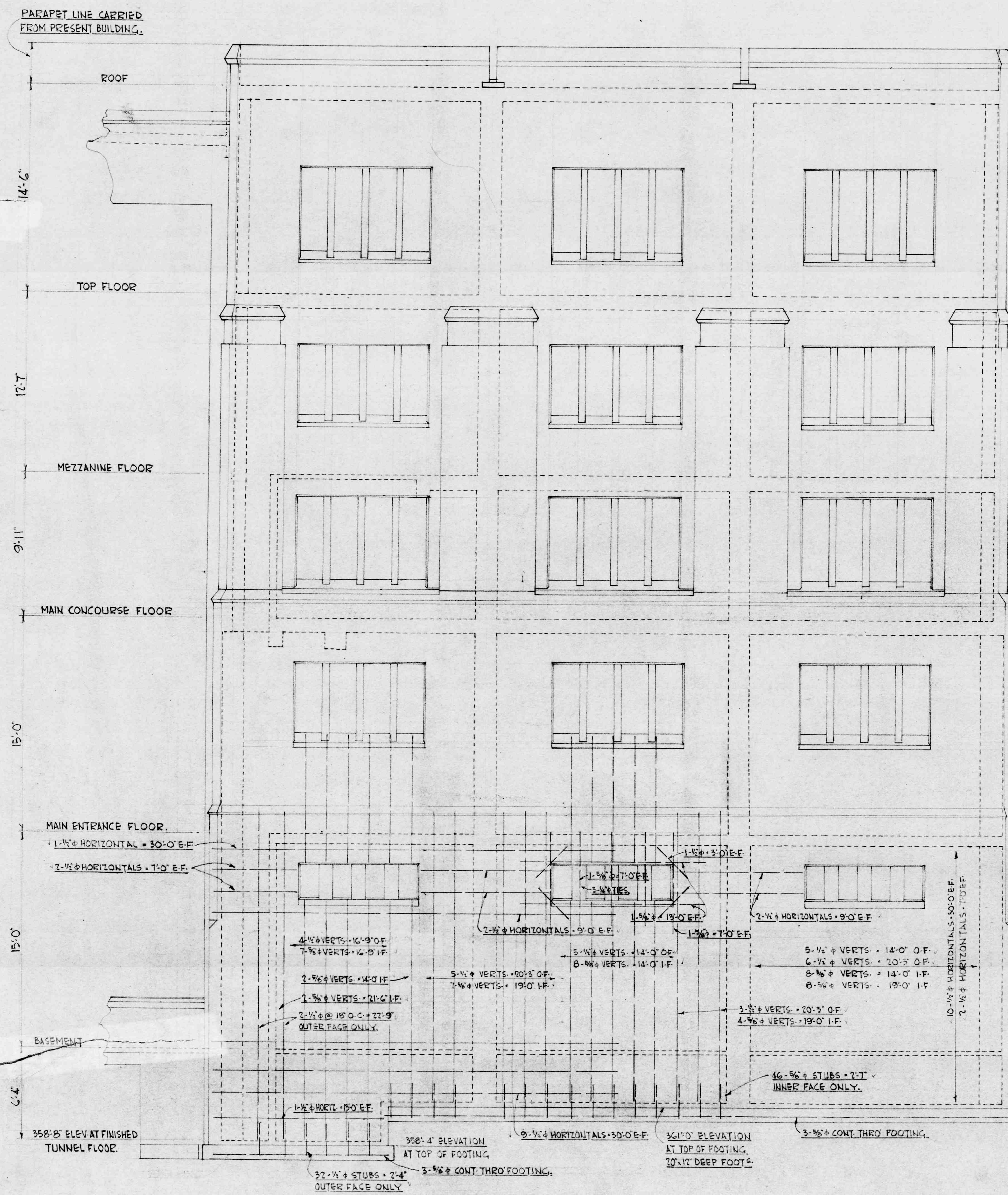
REAR (EAST) ELEVATION
