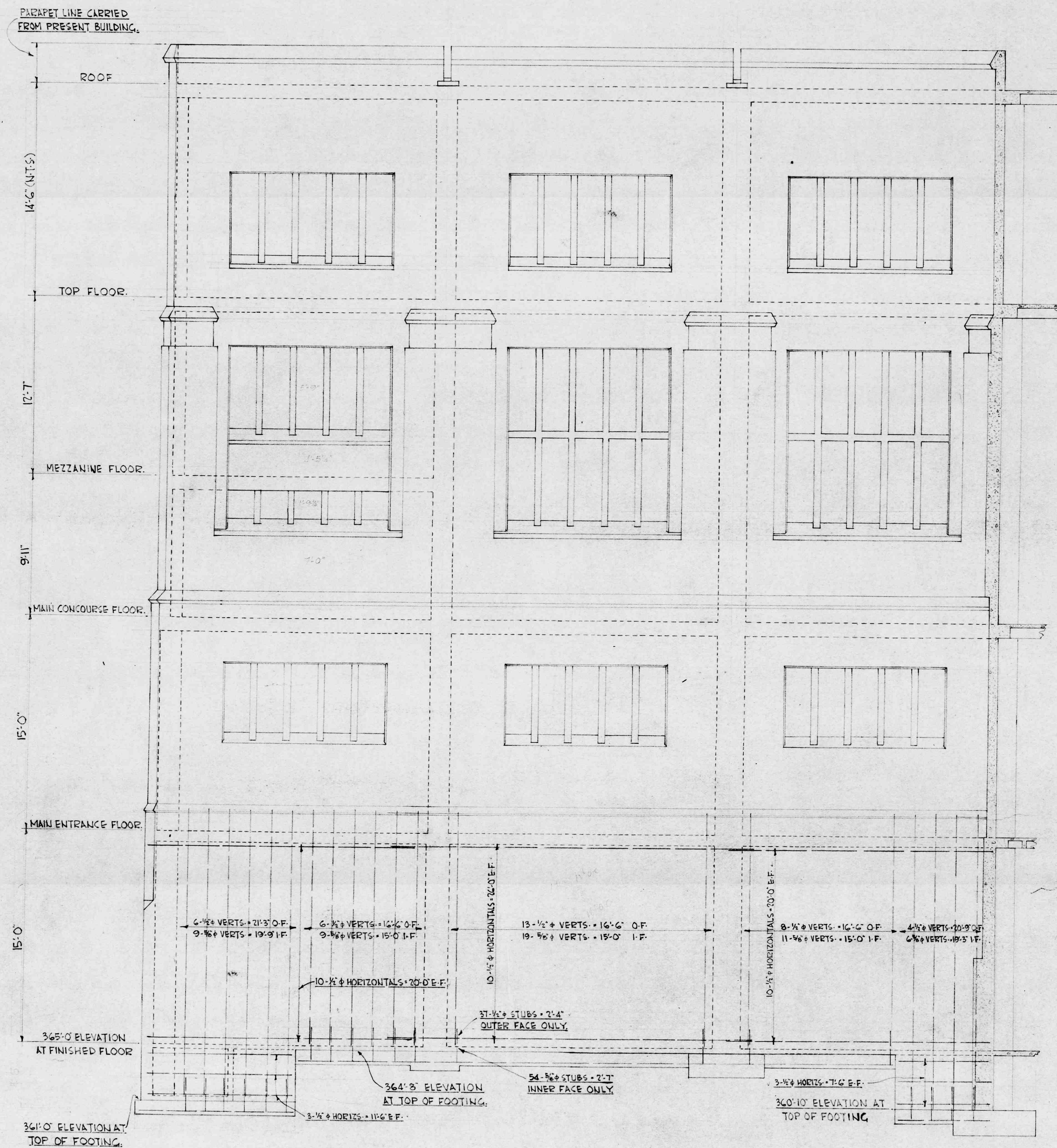
END (NORTH) ELEVATION
