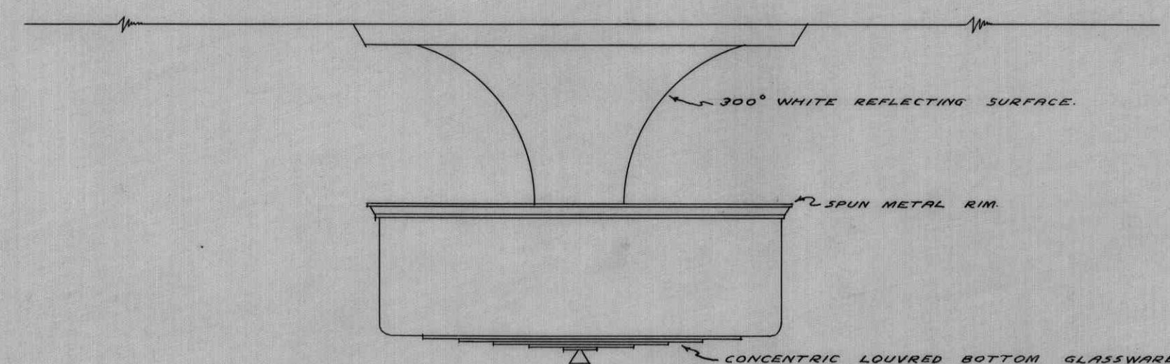
TYPE J" FIXTURE DETAIL SCALE - 1/4"=1"
