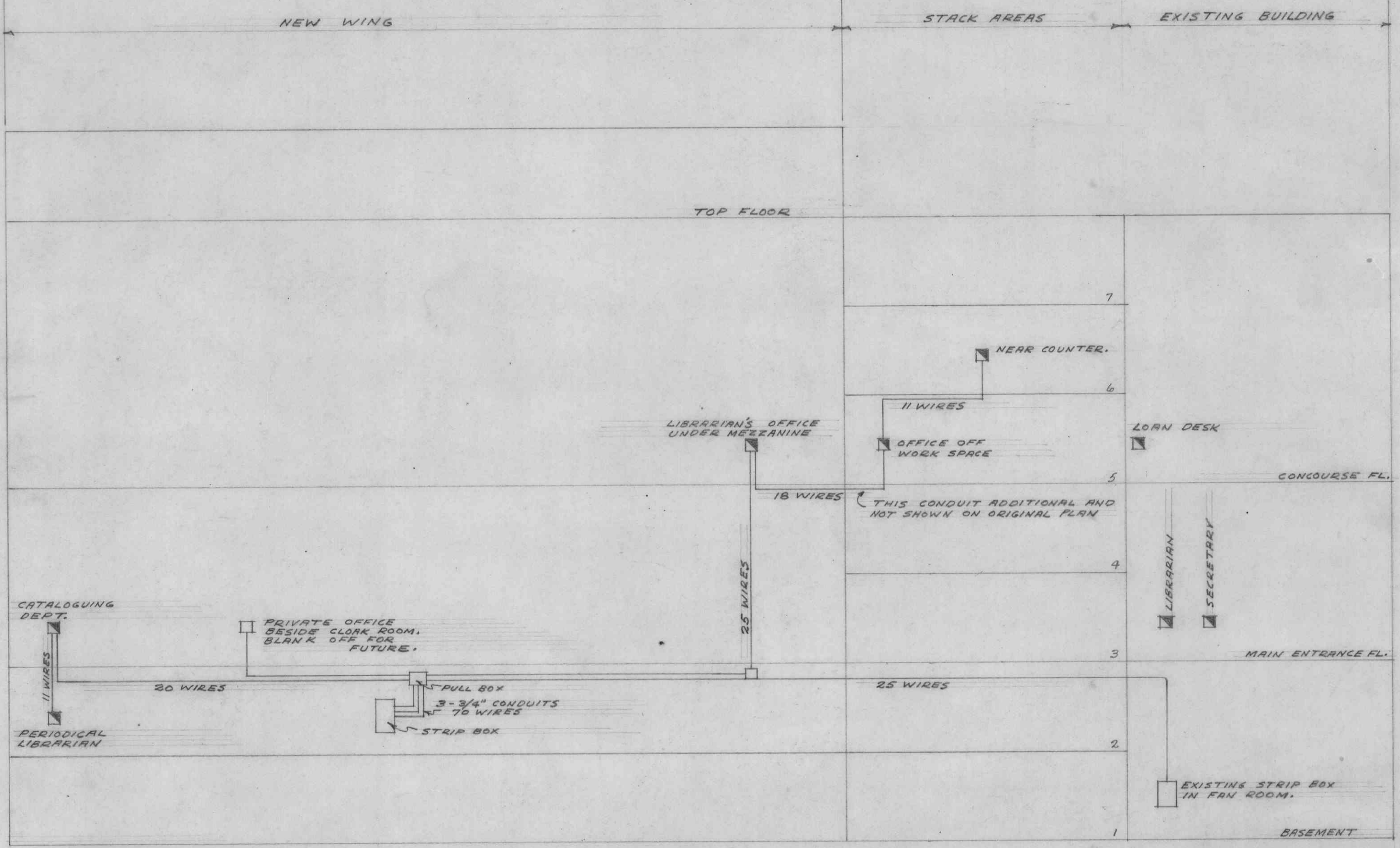
RISER DIAGRAM INTER-COMMUNICATION SYSTEM NOT TO SCALE
