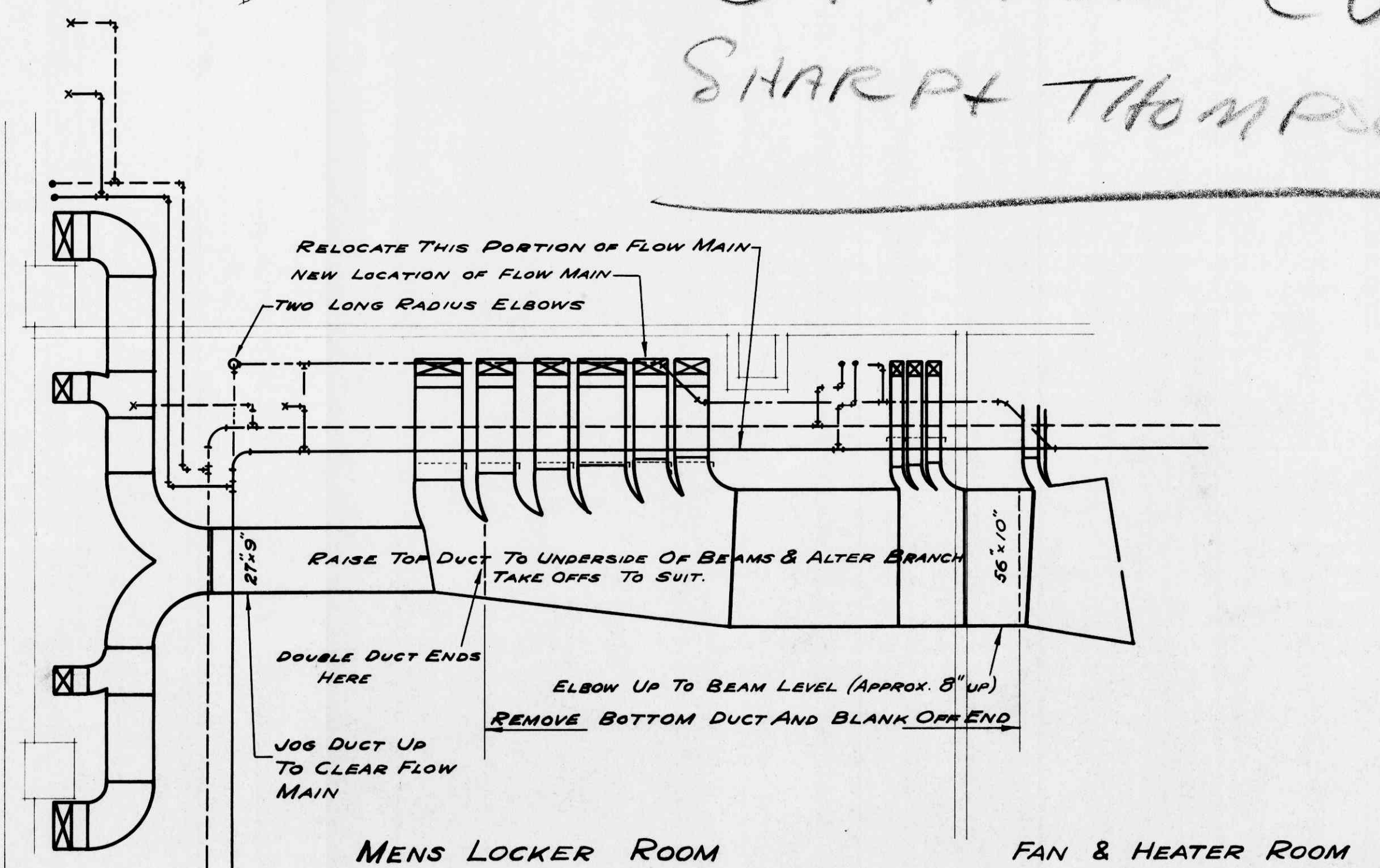
DETAIL OF ALTERATIONS TO PRESENT PIPING & DUCTWORK.
