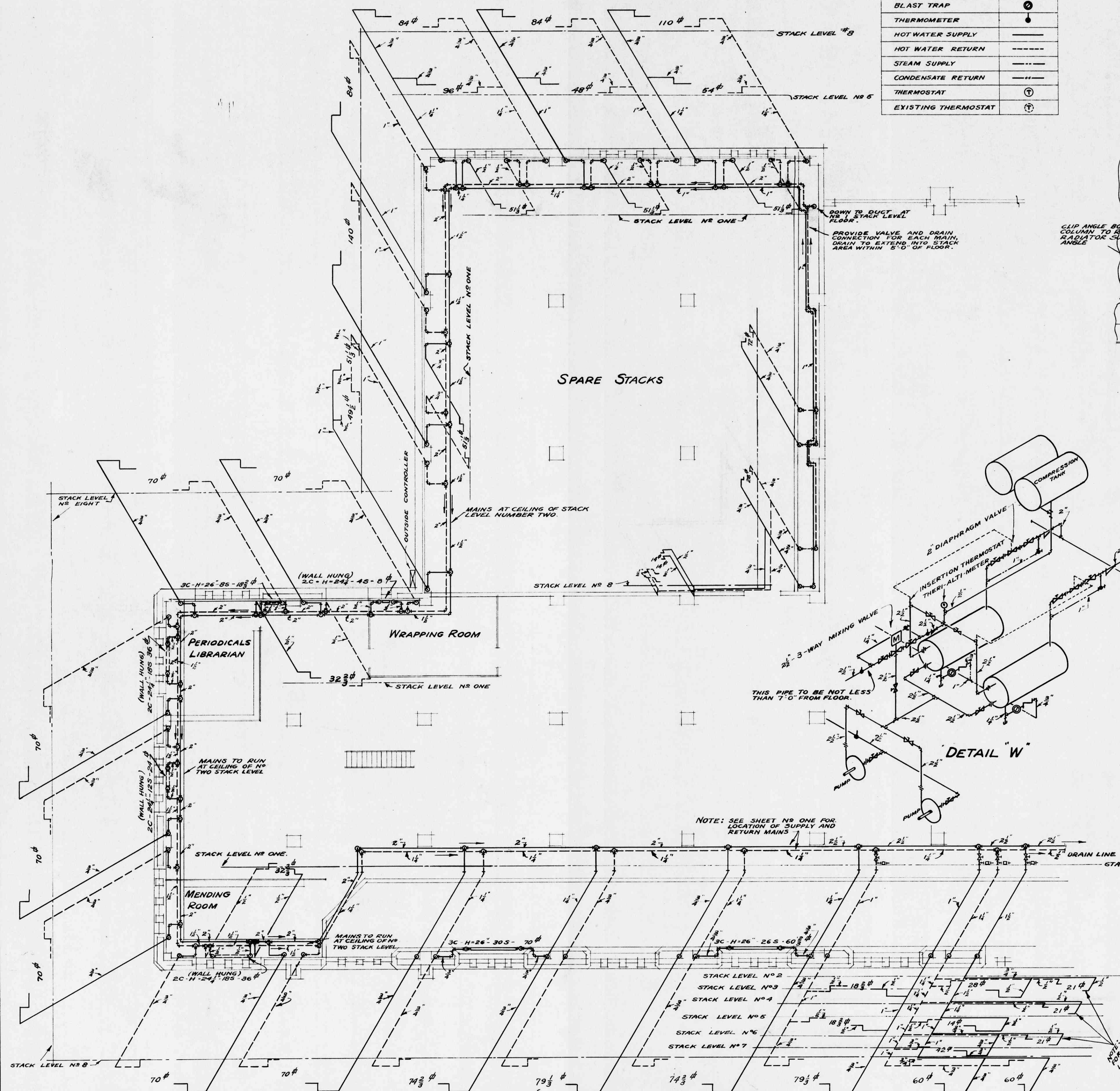
SCALE \frac{1}{8}'' = 1'-0''
