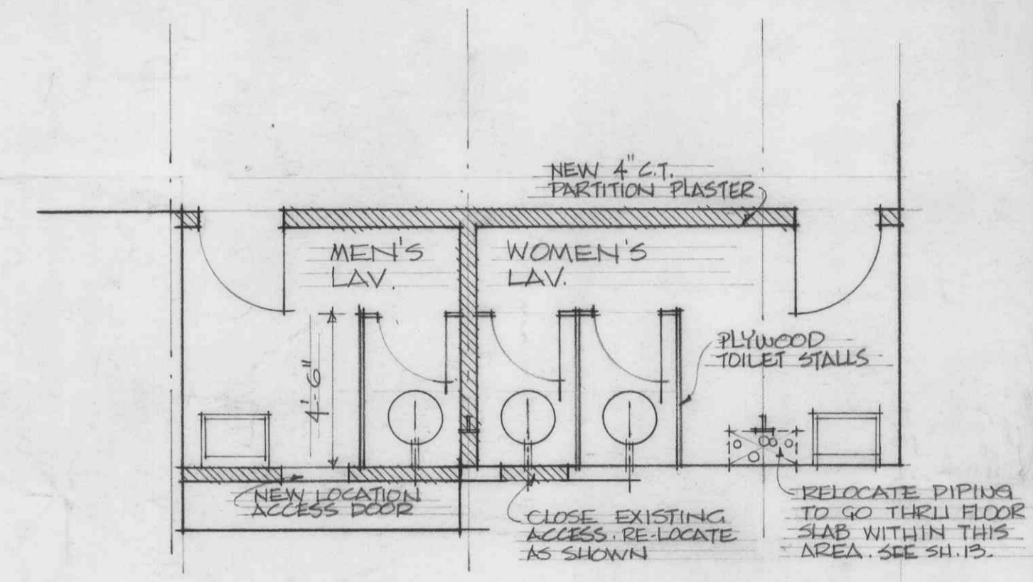
PLAN OF NEW LAVS SCALE 1/4" = 1'-0"
