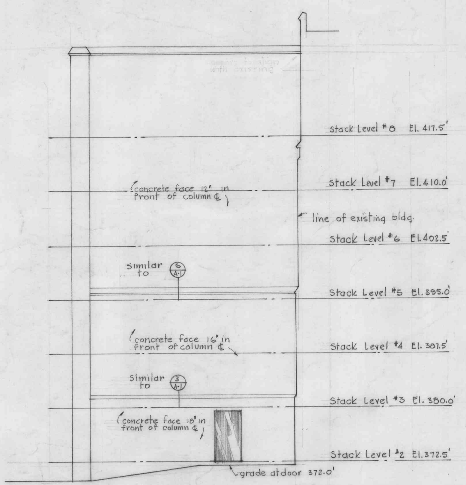
NORTH ELEVATION FOR ELEVATION USED IN ALTERNATE #1 SEE SHT. A-9
