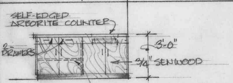
ONE SHELF (FIXED) SINK-UNIT RM# 821
