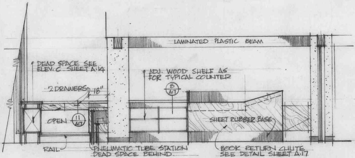
ELEVATION (K) (SEE PAGE 2 ADDENDUM NO. 2) SCALE: 1/4" = 1'-0"
