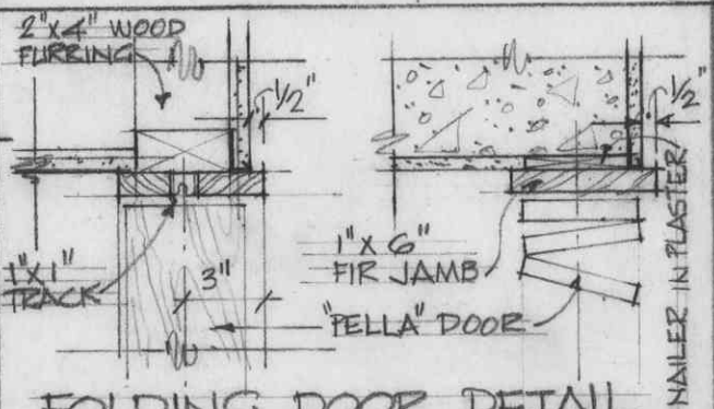
FOLDING DOOR DETAIL IN ROOM NO. 701
