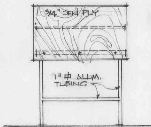
REAR ELEVATION
