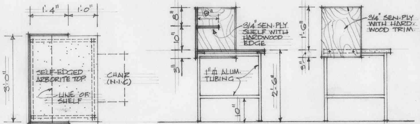
SECTION
