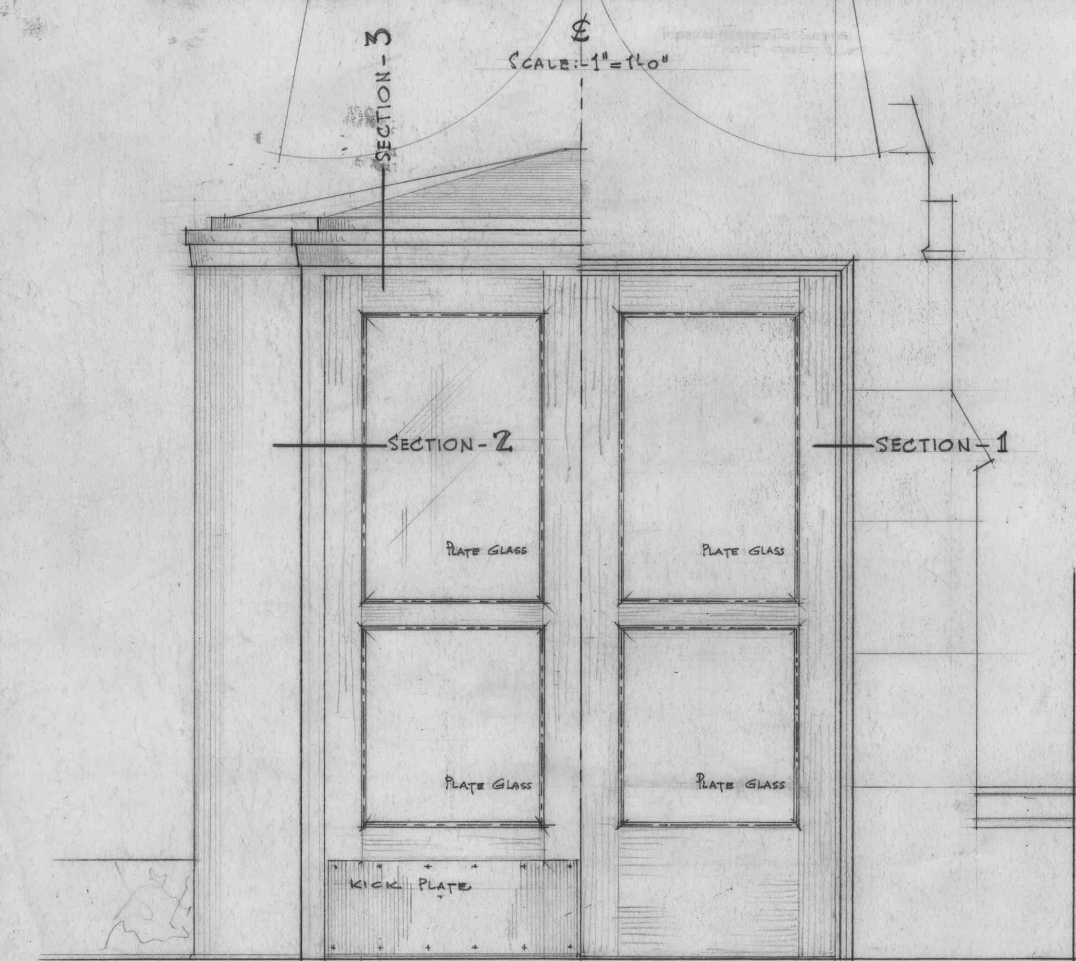
HALF INTERIOR ELEV. HALF EXTERIOR ELEV. SCALE: 1" = 1'-0"
