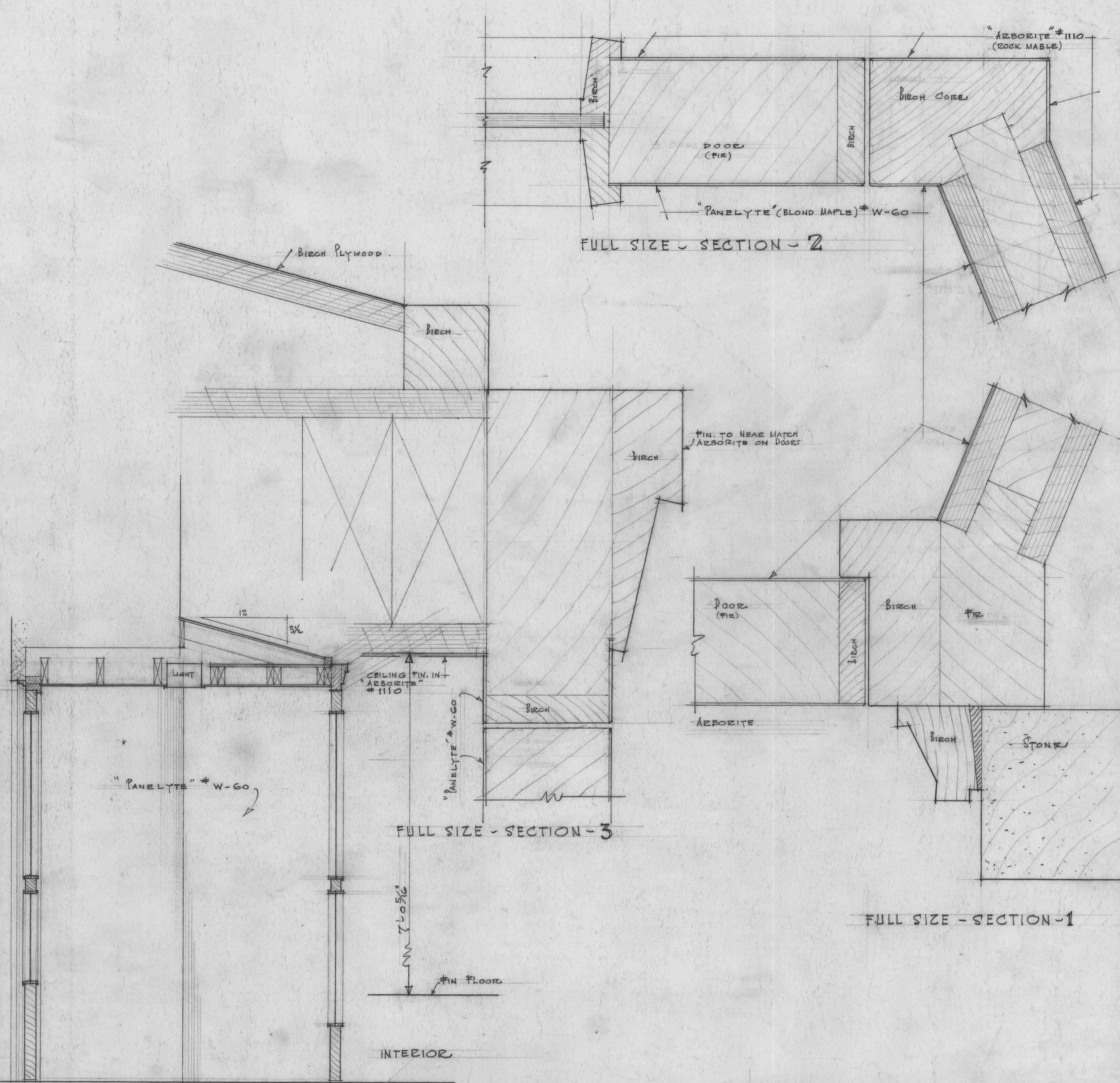
SECTION SCALE: 1" = 1'-0" FULL SIZE - SECTION-1 FULL SIZE - SECTION-2 FULL SIZE - SECTION-3 EXTERIOR INTERIOR
